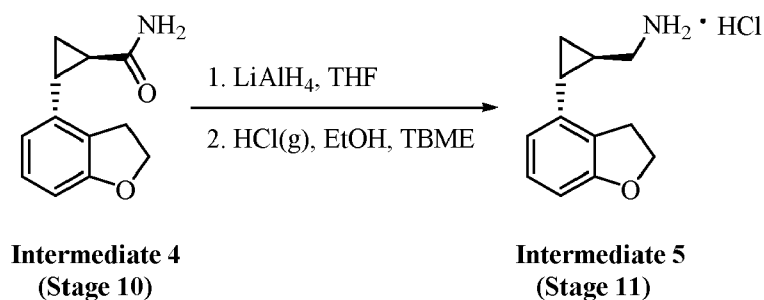
[Scheme 5]
