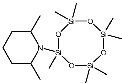
2-(2,6-dimethylpiperidino)-2,4,4,6,6,8,8-heptamethylcyclotetrasiloxane
