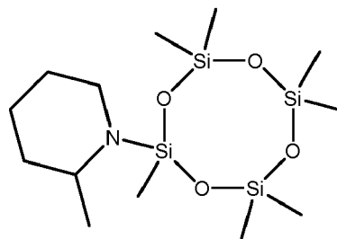
2-(2-methylpiperidino)-2,4,4,6,6,8,8-heptamethylcyclotetrasiloxane
