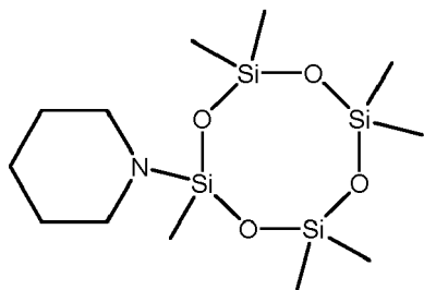
2-piperidino-2,4,4,6,6,8,8-heptamethylcyclotetrasiloxane
