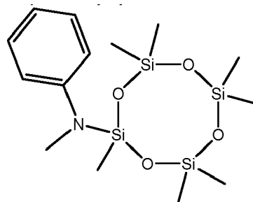
2-phenylmethylamino-2,4,4,6,6,8,8-heptamethylcyclotetrasiloxane
