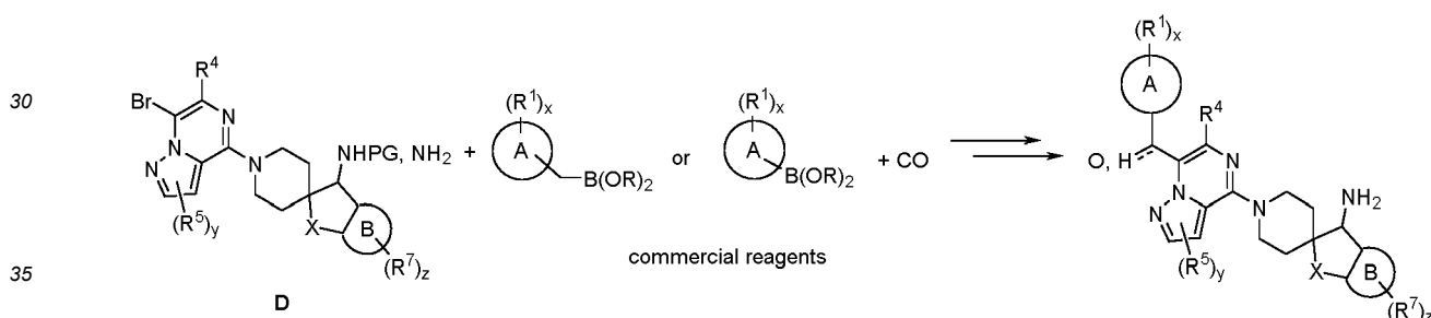
Scheme 2.
