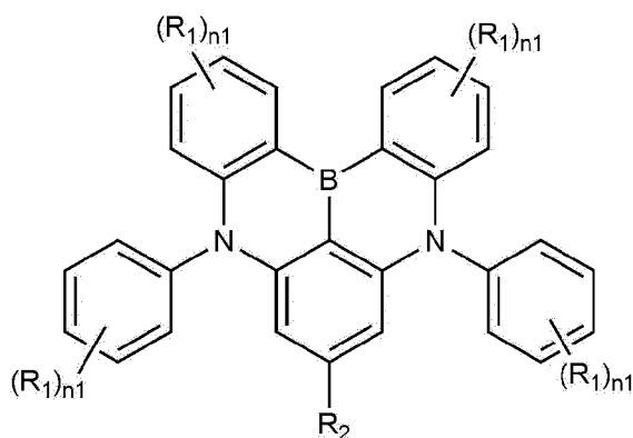
[Chemical Formula 1]
