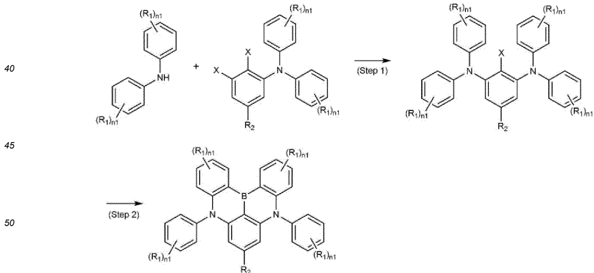
[Reaction Scheme 1]
