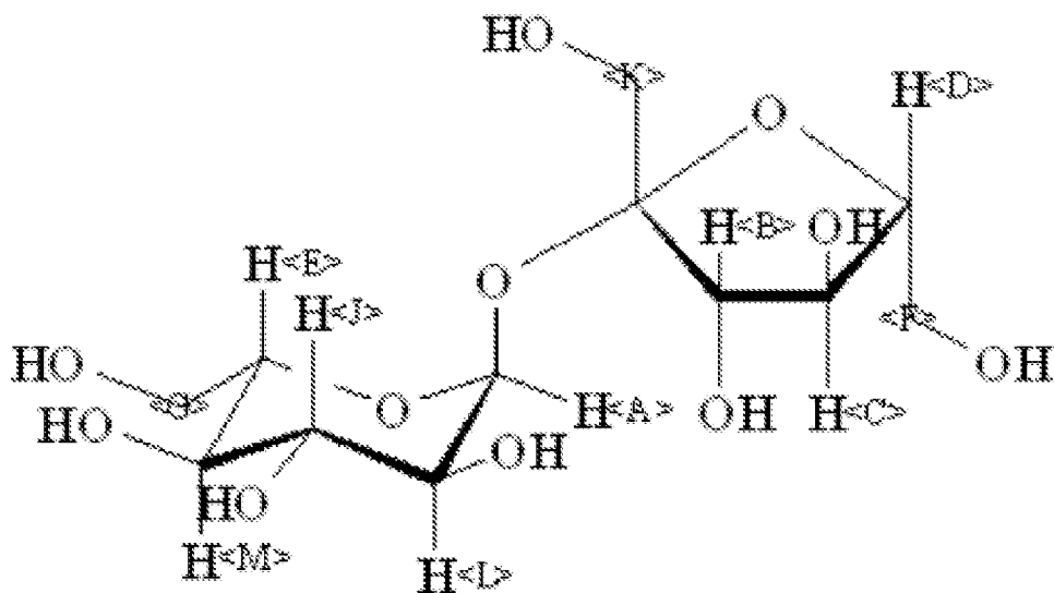
Formula (I)
