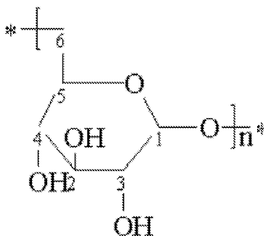
Formula (III)
