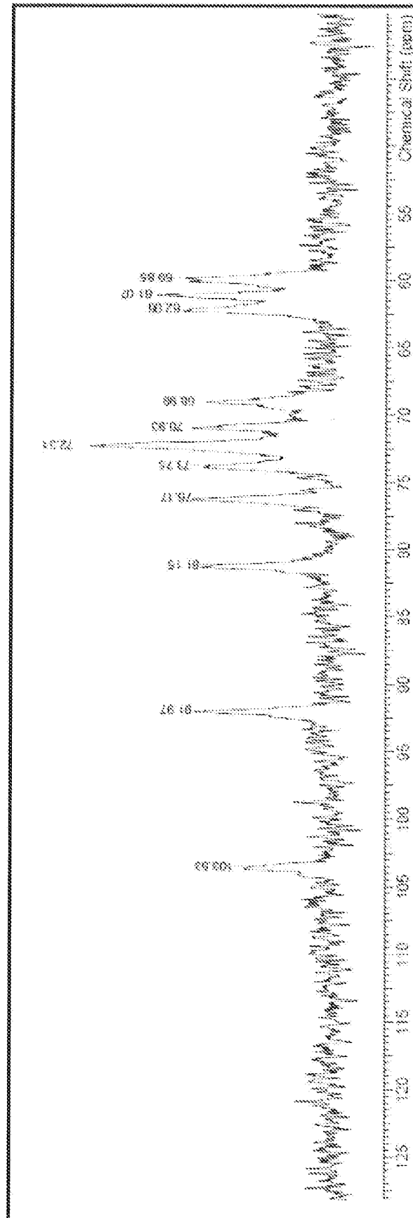
FIG. 20: ^{13}\text{C} NMR spectra of S2-preparation 1
