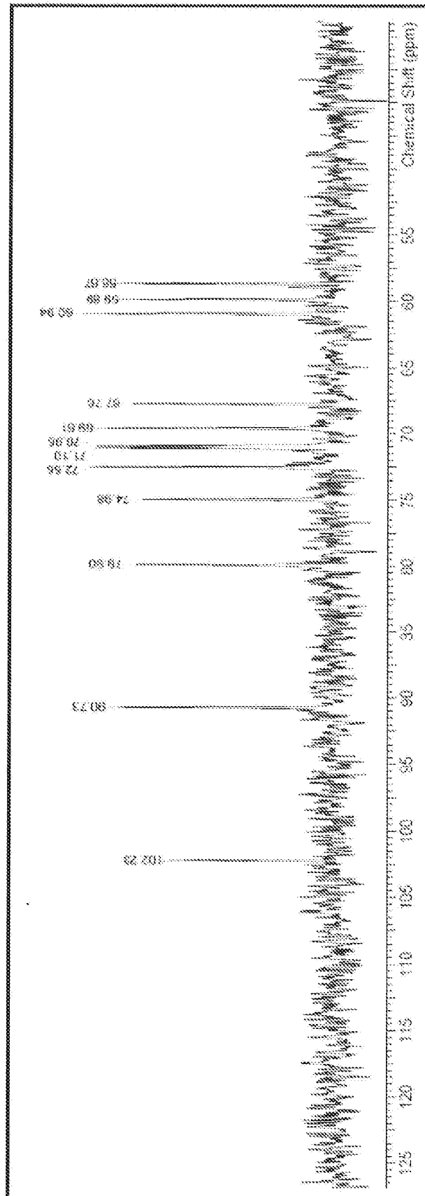
FIG. 19: ^{13}\text{C} NMR spectra of S1-preparation 1
