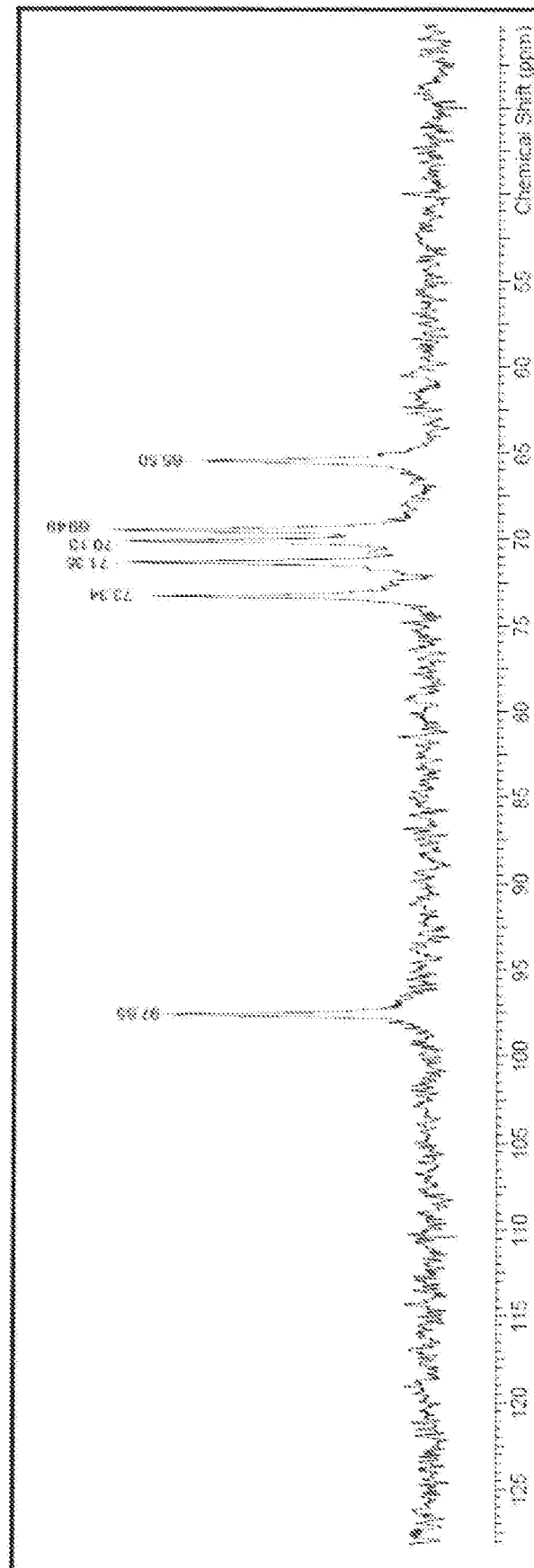
FIG. 21: ^{13}\text{C} NMR spectra of S3-preparation 1
