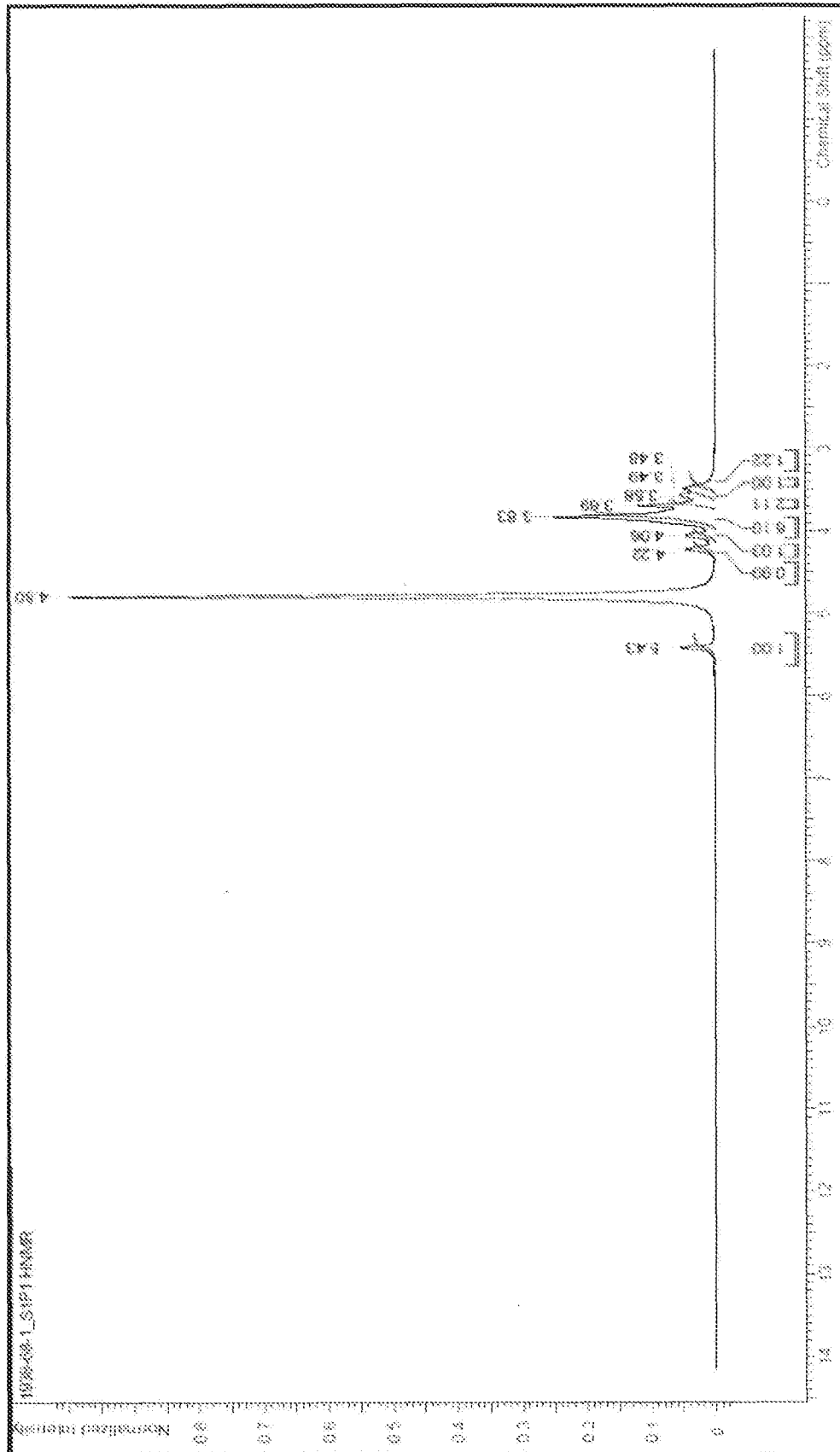
FIG. 16: ^1\text{H} NMR spectra of S1-preparation 1
