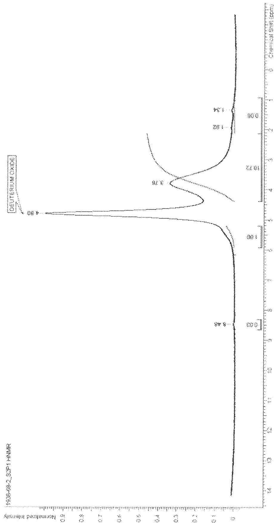
FIG. 17: ^1\text{H} NMR spectra of S2-preparation 1
