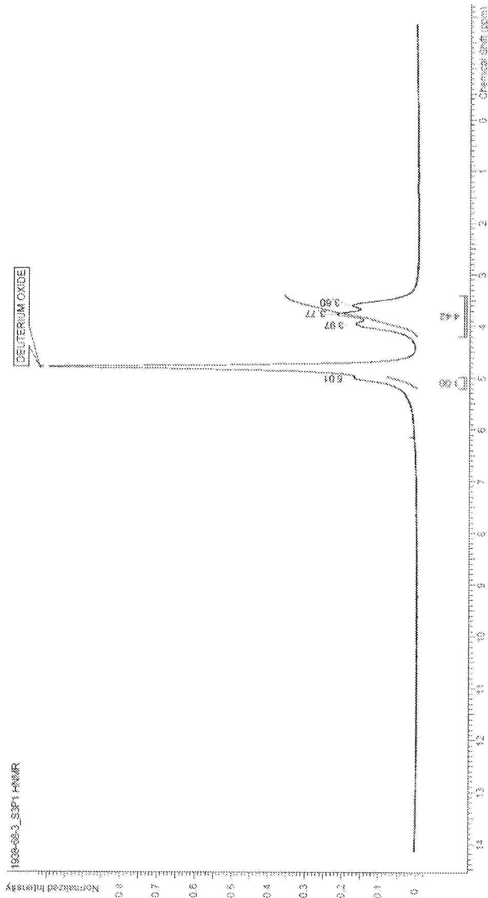
FIG. 18: ^1\text{H} NMR spectra of S3-preparation 1
