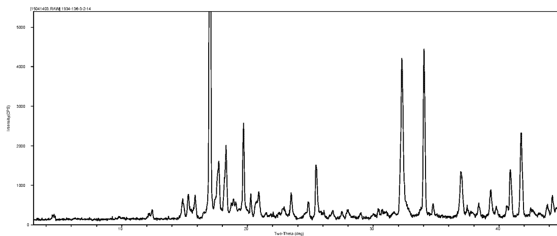
FIG. 16 XRPD Form X
