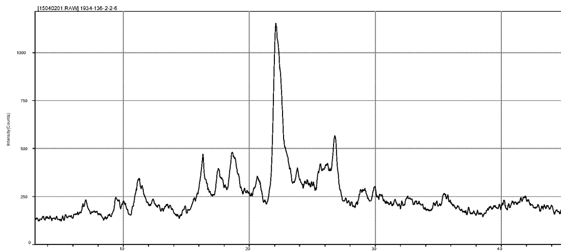
FIG. 9 XRPD Form IV
