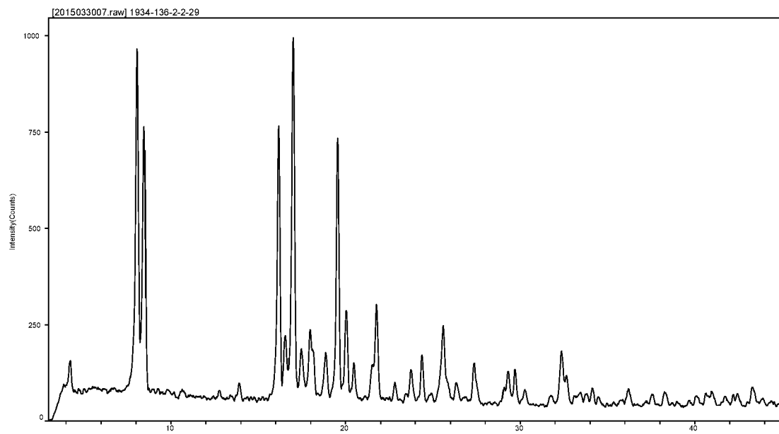
FIG. 14 XRPD Form VIII
