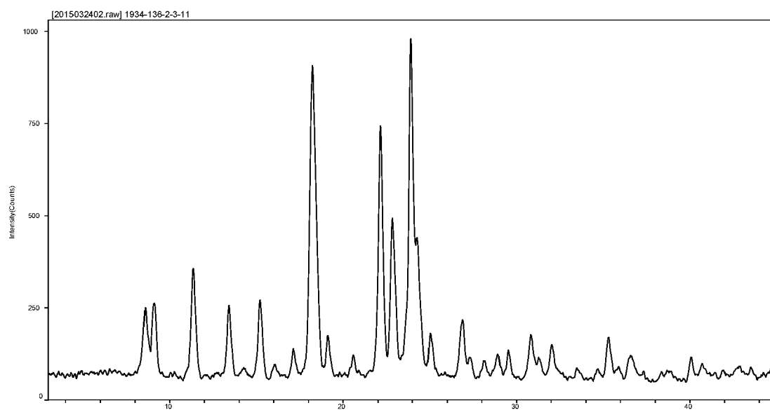
FIG. 15 XRPD Form IX
