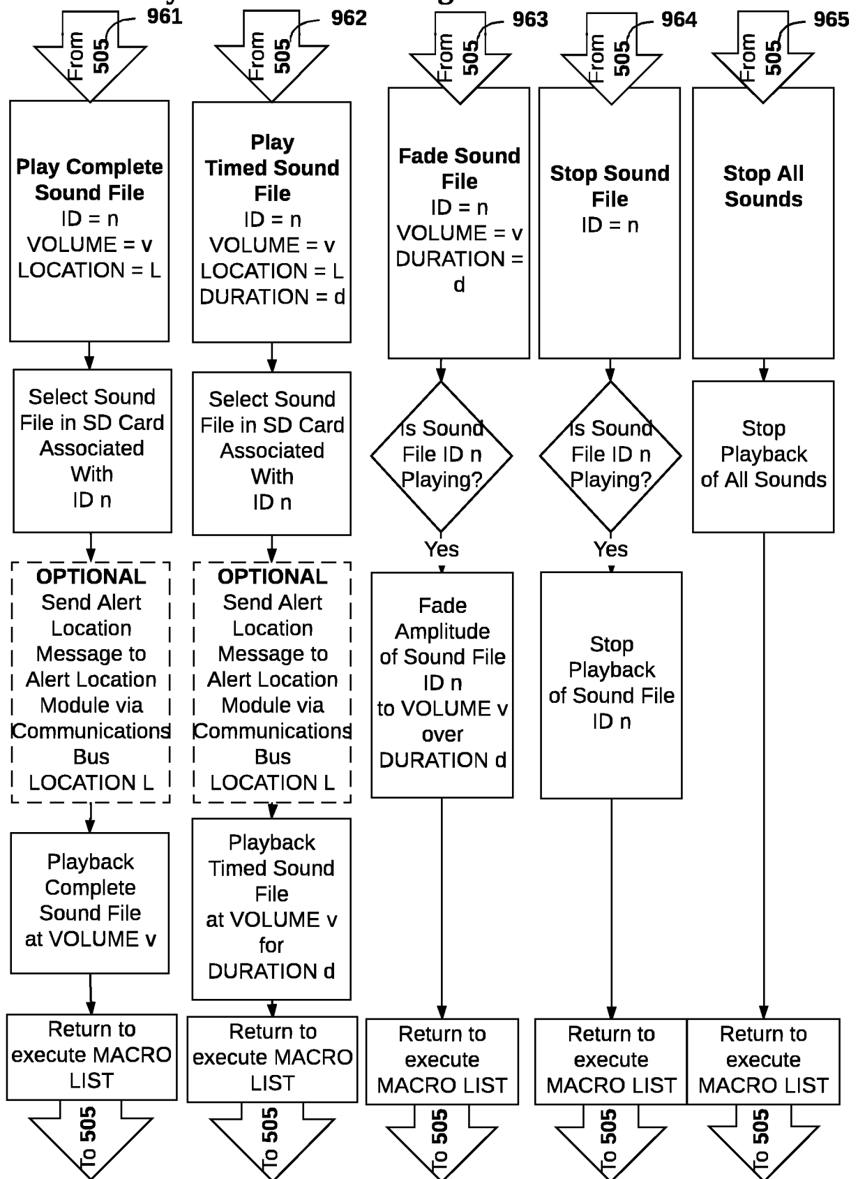
FIG. 9A - System Behaviors Logic Flow
