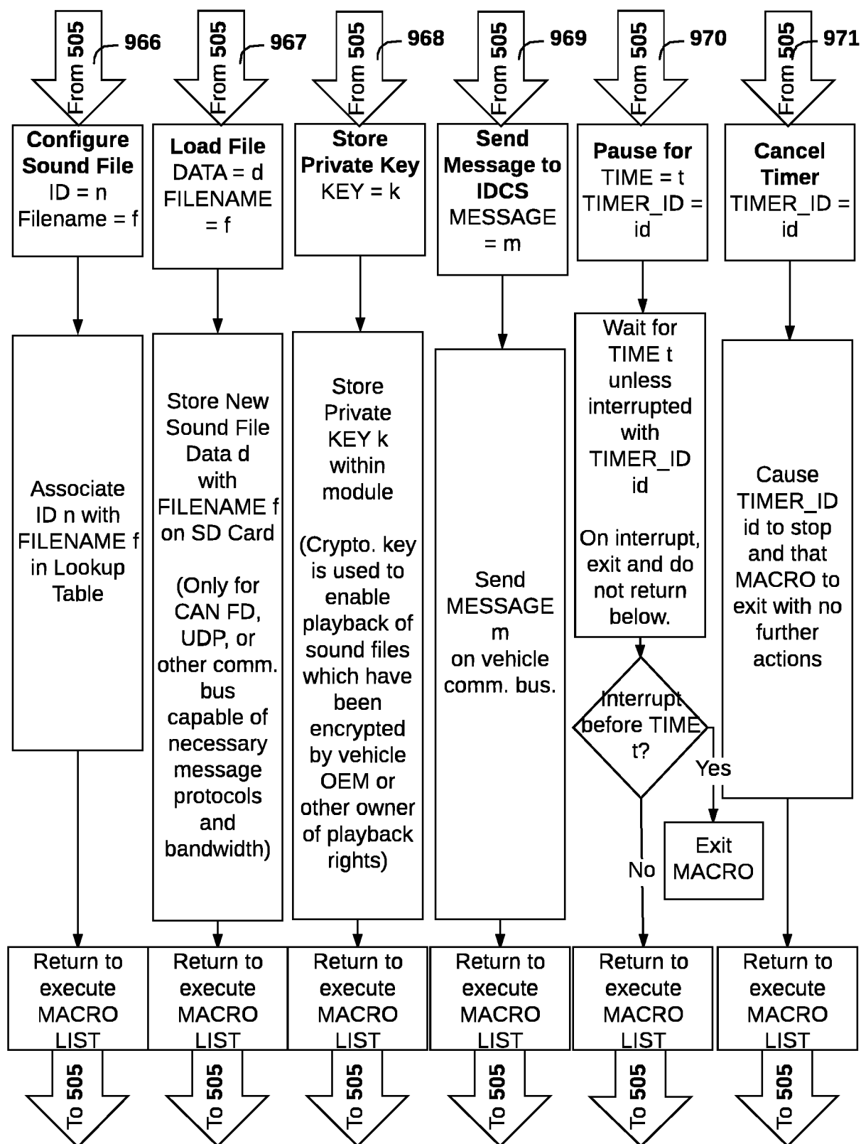
FIG. 9B - System Behaviors Logic Flow
