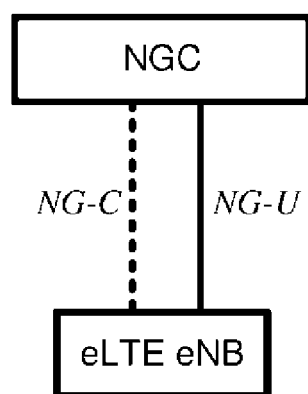
FIG. 10B eLTE eNB connected to NGC
