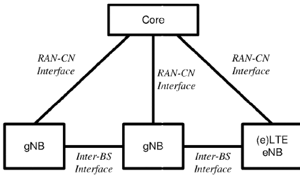
FIG. 13A Non-centralized deployment
