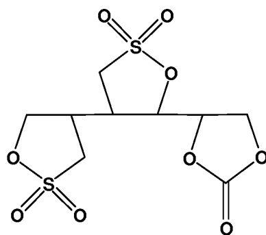
Compound 13
