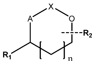
Structure formula 1
