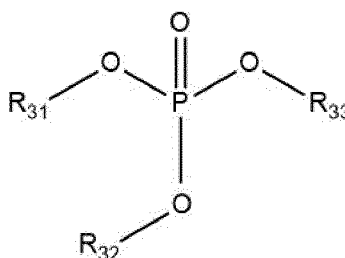
Structure formula 3
