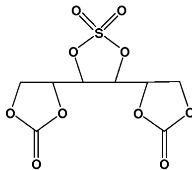
Compound 8
