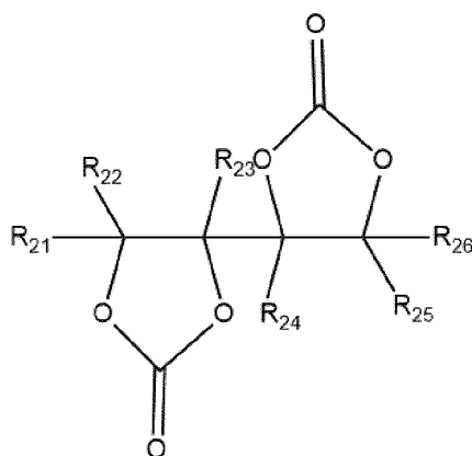
Structure formula 2
