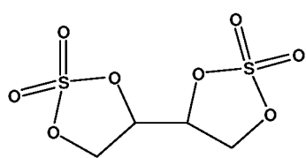
Compound 4
