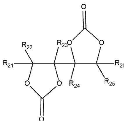
Structure formula 2
