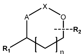
Structure formula 1
