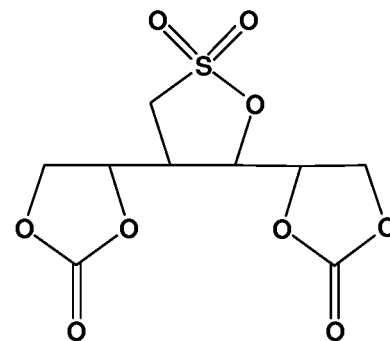
Compound 12
