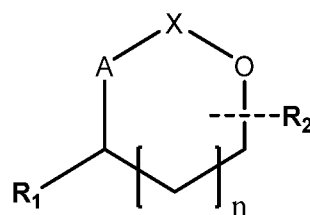
Structure formula 1
