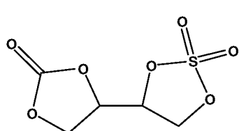
Compound 1
