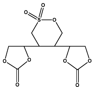
Compound 15
