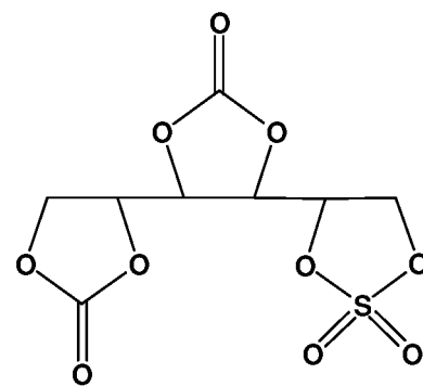
Compound 10
