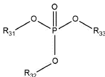
Structure formula 3
