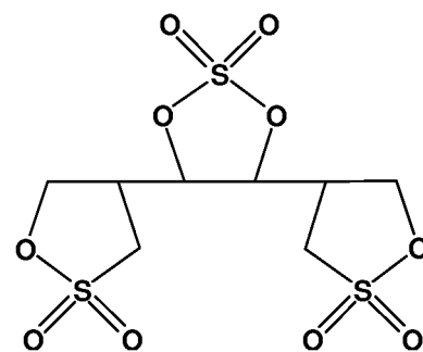
Compound 16
