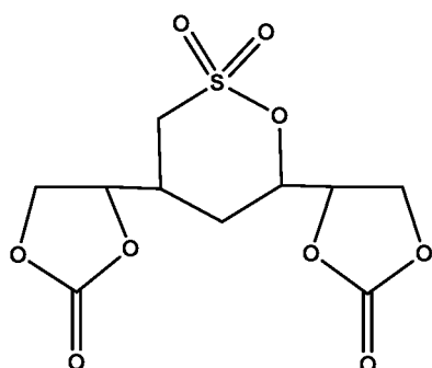
Compound 19
