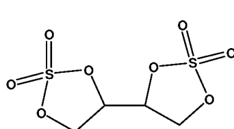
Compound 4
