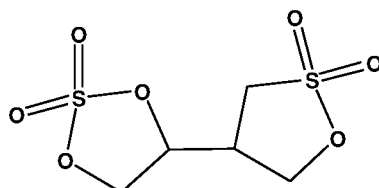
Compound 5
