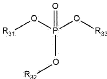
Structure formula 3
