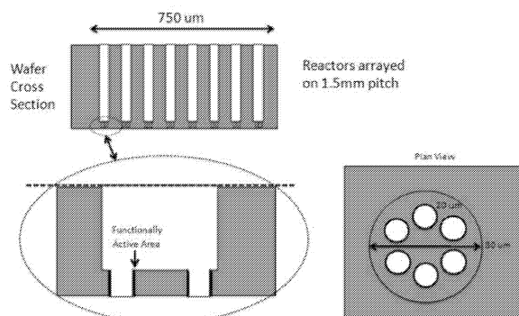
Figure 4 Oligo Wafer Reactor
