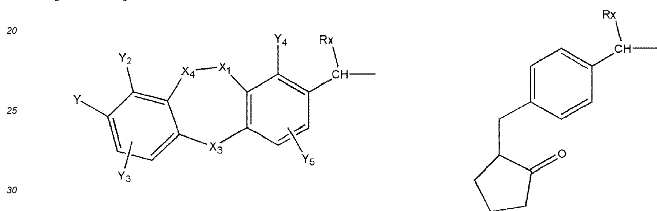
[Chem.49]
