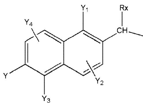
[Chem.42]
