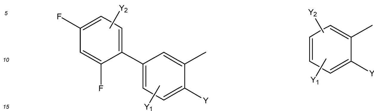
[Chem.58]
