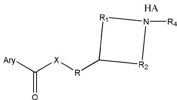
Structure 2b
