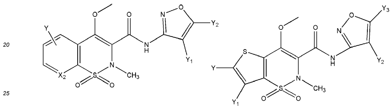
[Chem.31]
