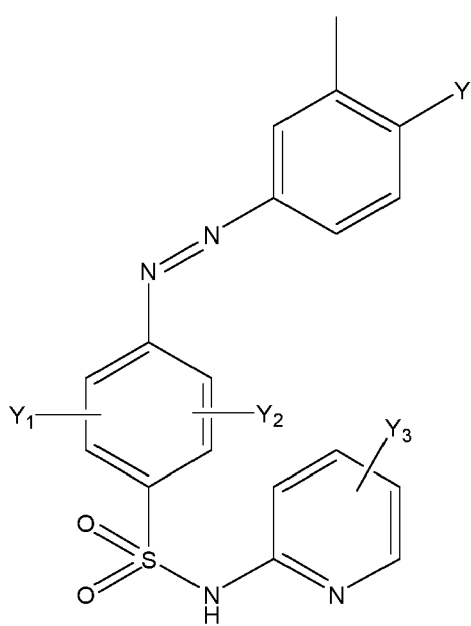
[Chem.61]
