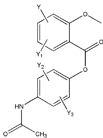
[Chem.29]
