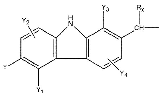
[Chem.44]
