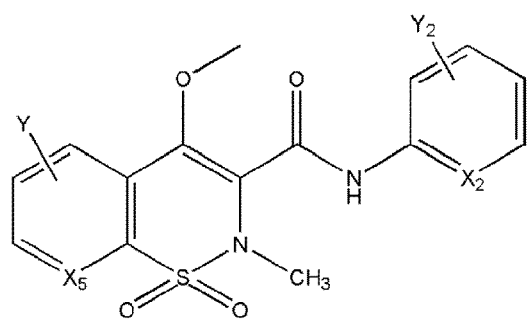
[Chem.69]
