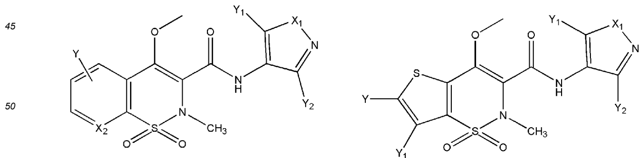
[Chem.33]
