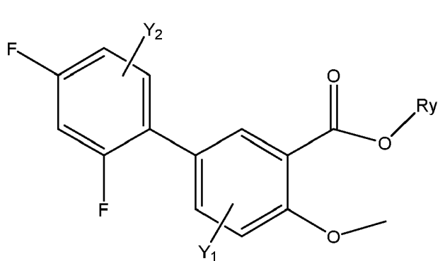
[Chem.62]
