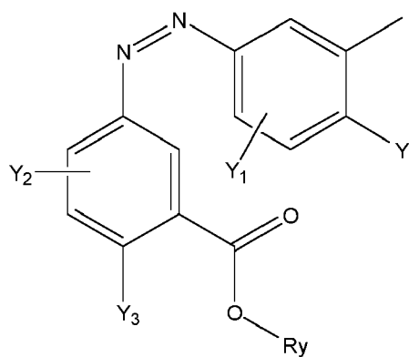
[Chem.68]
