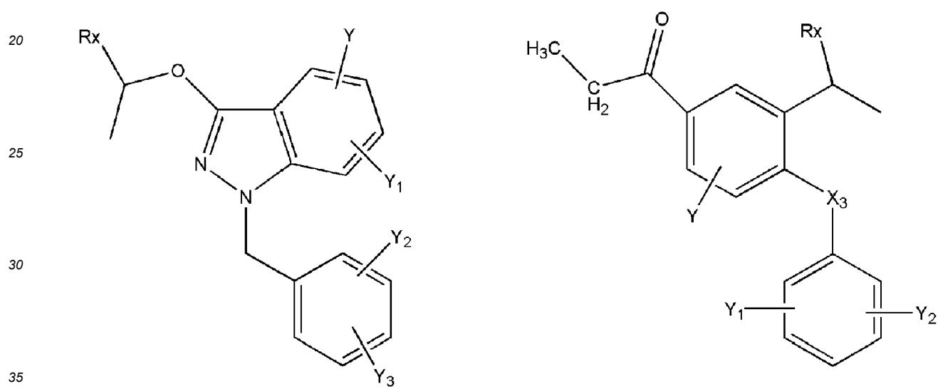
[Chem.58]
