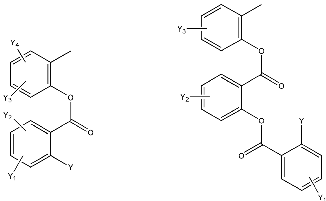
[Chem.20]
