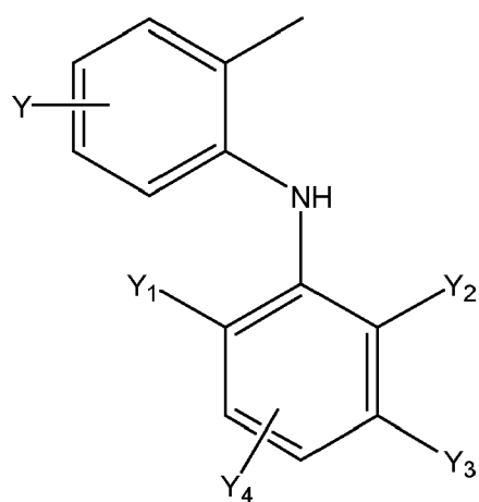
[Chem.63]
