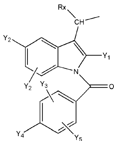
[Chem.4]
