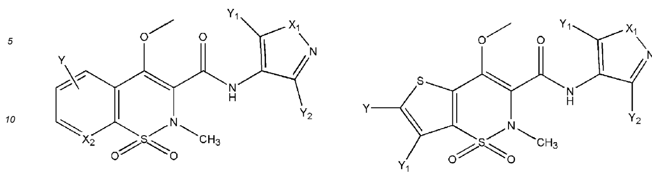
[Chem.72]
