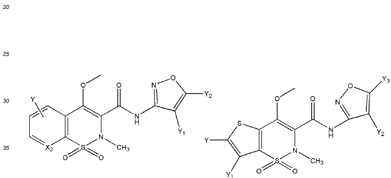
[Chem.71]
