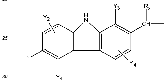
[Chem.44]
