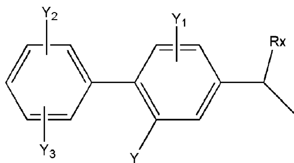
[Chem.65]
