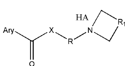
Structure 2c
