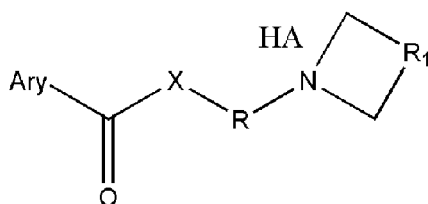
Structure 2c
