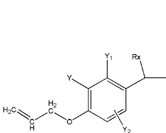
[Chem.16]
