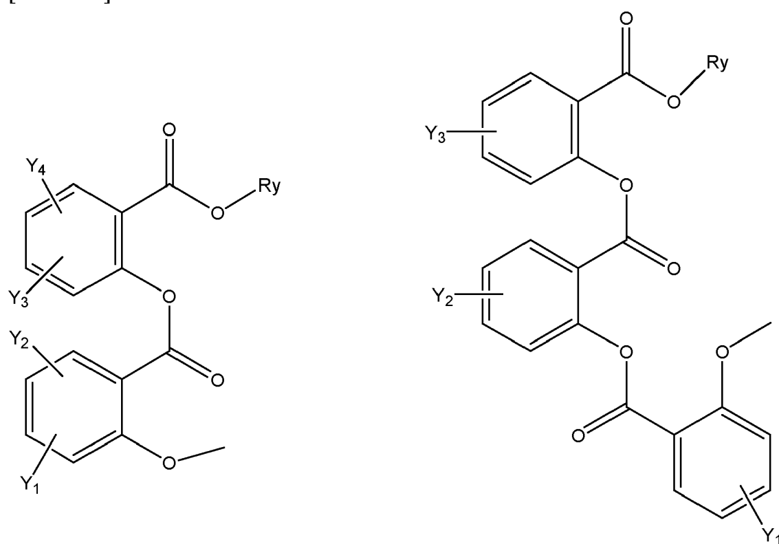
[Chem.62]
