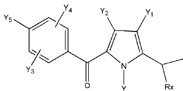
[Chem.53]
