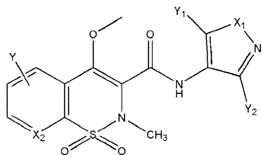
[Chem.72]
