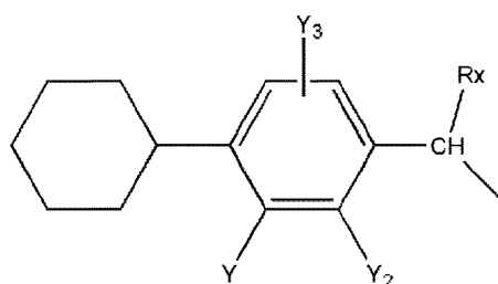
[Chem.46]
