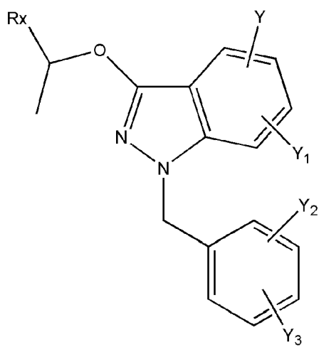
[Chem.19]
