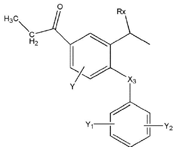
[Chem.59]
