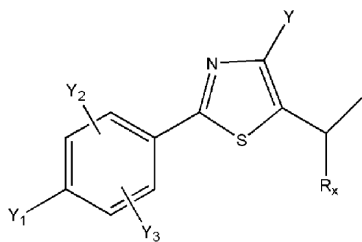
[Chem.56]
