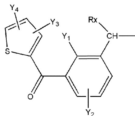
[Chem.42]
