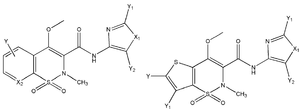
[Chem.36]
