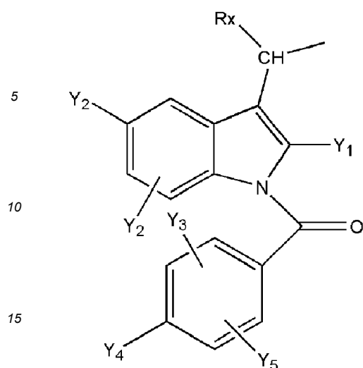
[Chem.44]
