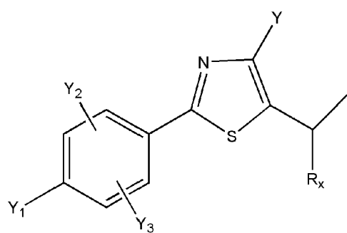
[Chem.17]
