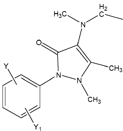
[Chem.66]
