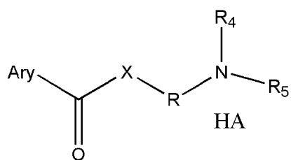
Structure 1
