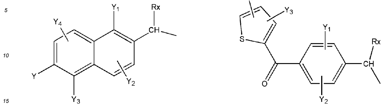
[Chem.42]
