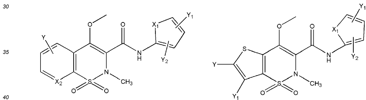
[Chem.32]
