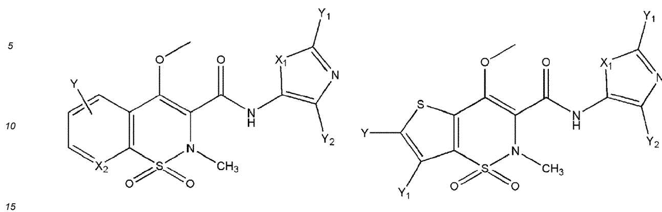
[Chem.75]
