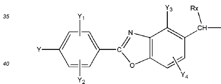
[Chem.45]
