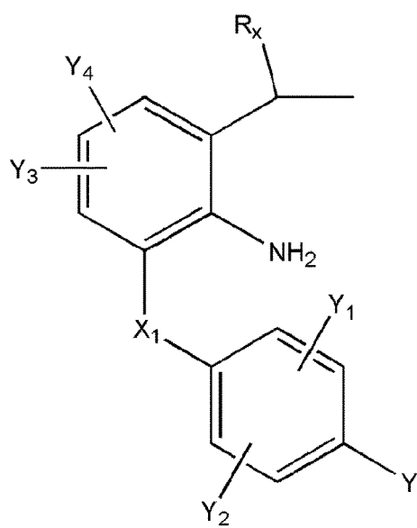
[Chem.55]
