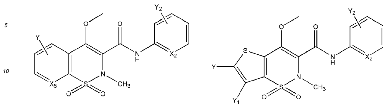
[Chem.69]
