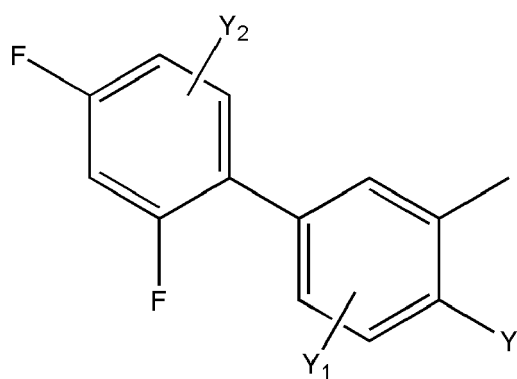
[Chem.18]
