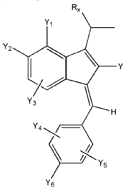
[Chem.52]
