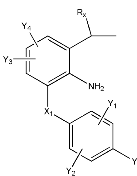
[Chem.15]
