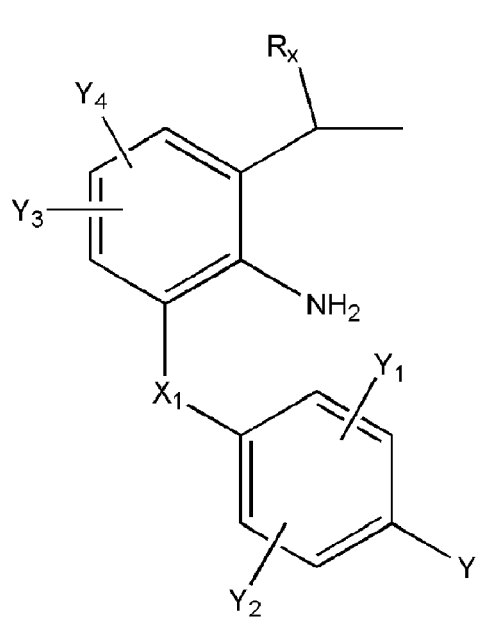
[Chem.55]
