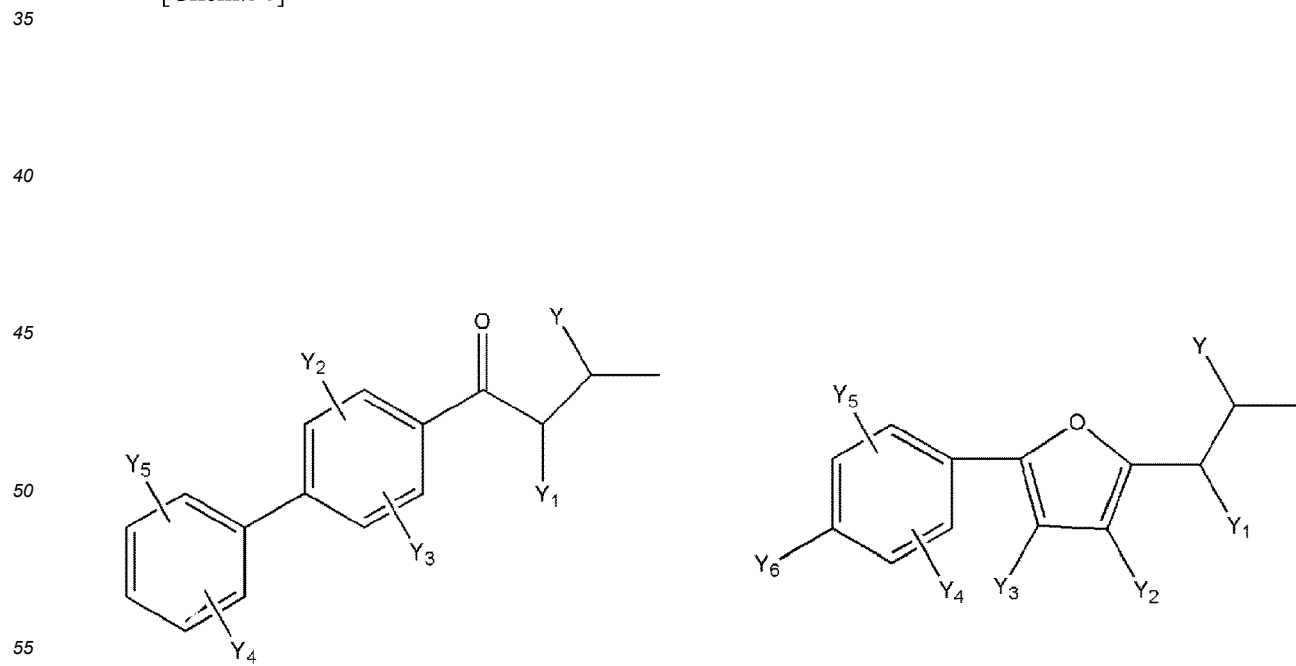
[Chem.51]
