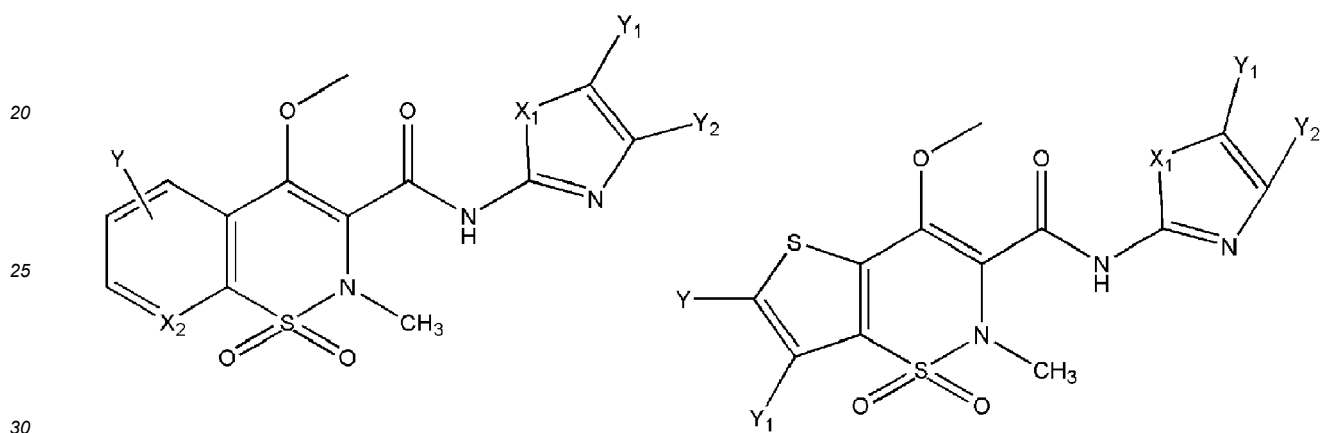
[Chem.73]
