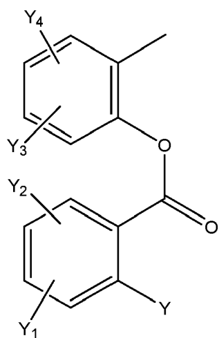
[Chem.60]
