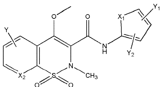
[Chem.71]
