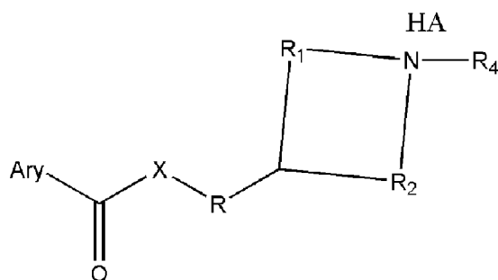
Structure 2b
