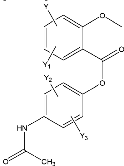
[Chem.68]
