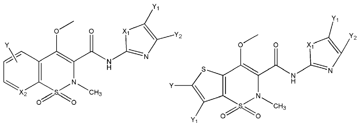
[Chem.34]
