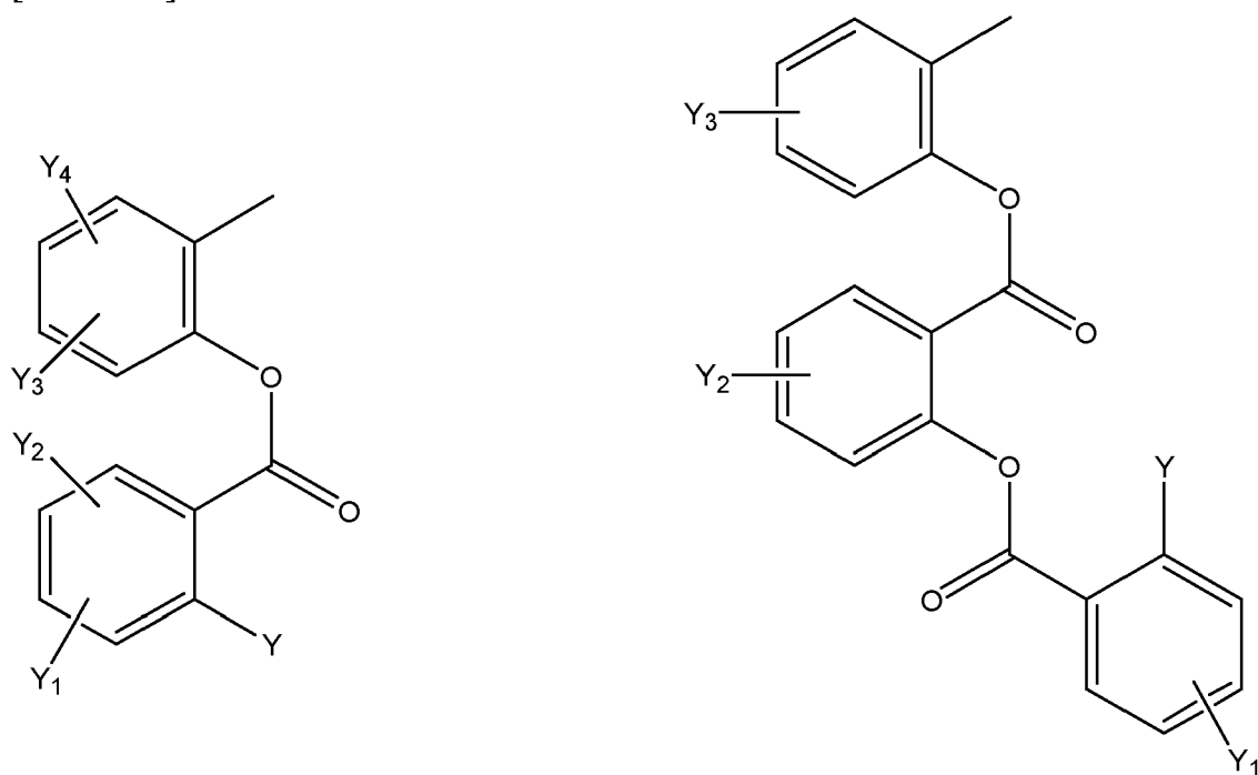
[Chem.59]
