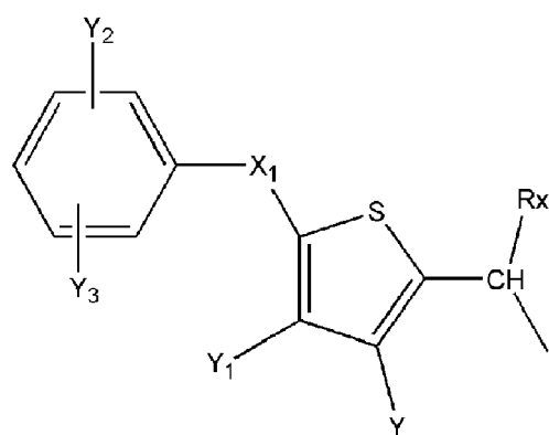
[Chem.48]
