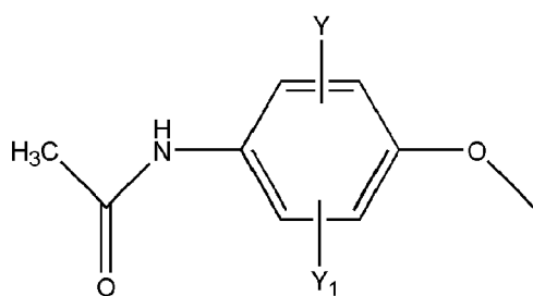
[Chem.25]
