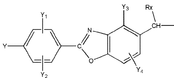
[Chem.45]
