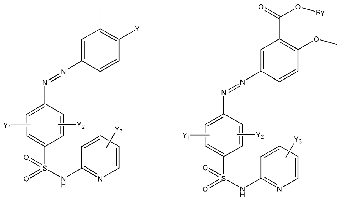
[Chem.21]
