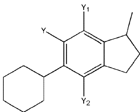
[Chem.52]
