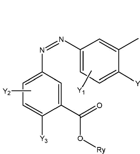
[Chem.68]
