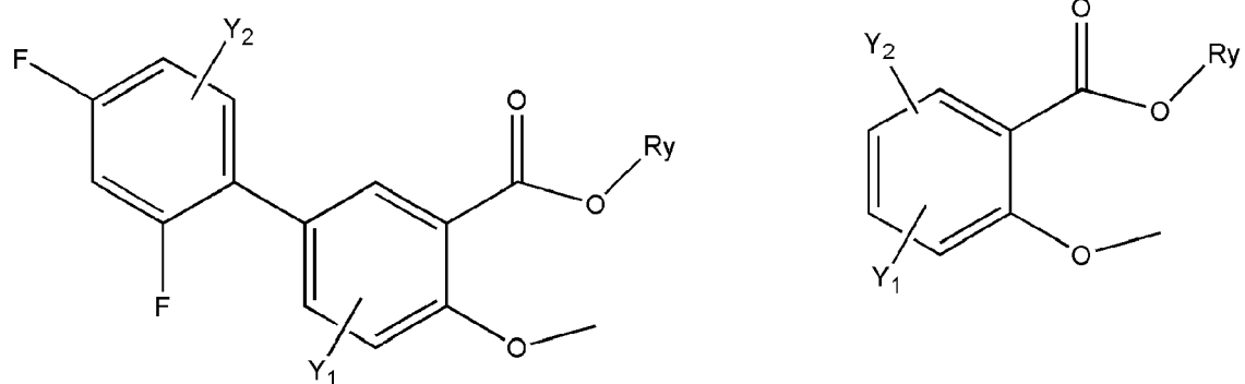
[Chem.22]
