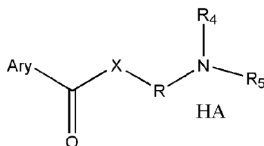
Structure 1
