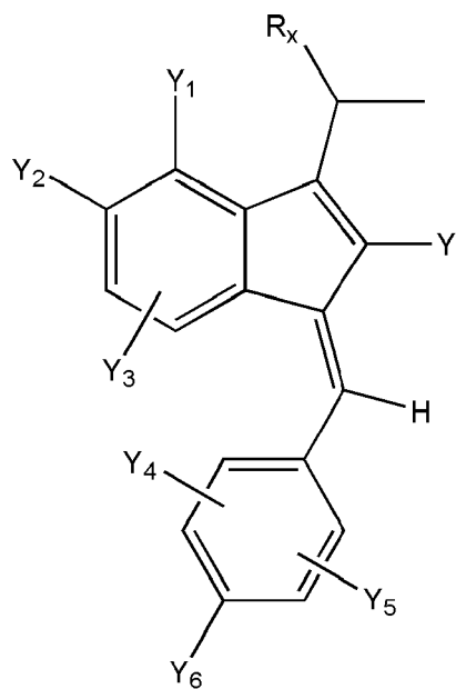
[Chem.13]
