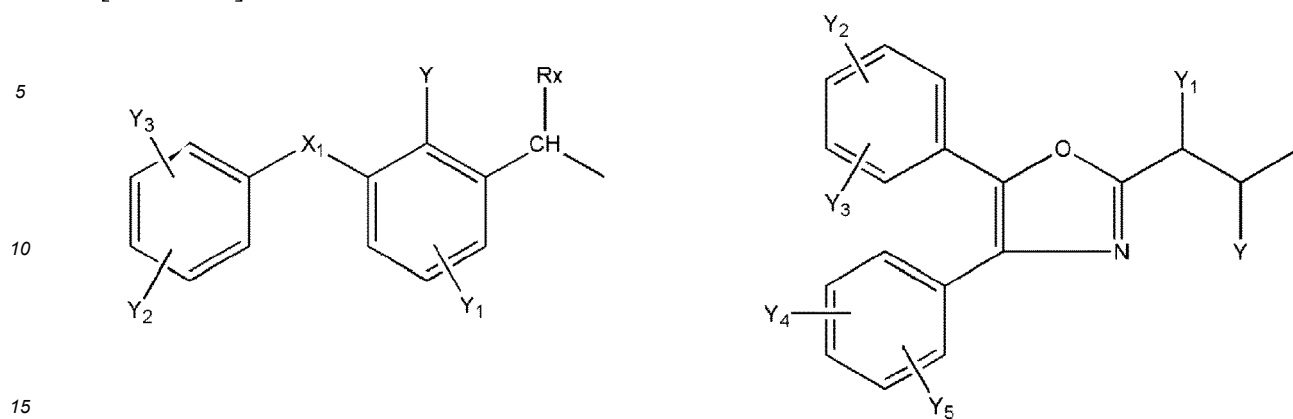
[Chem.48]
