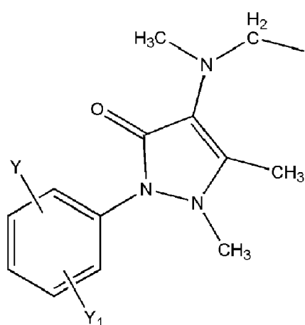
[Chem.66]
