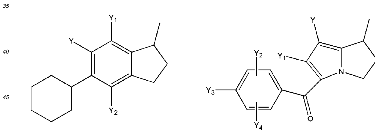
[Chem.51]
