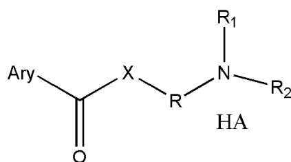
[Chem.1]
