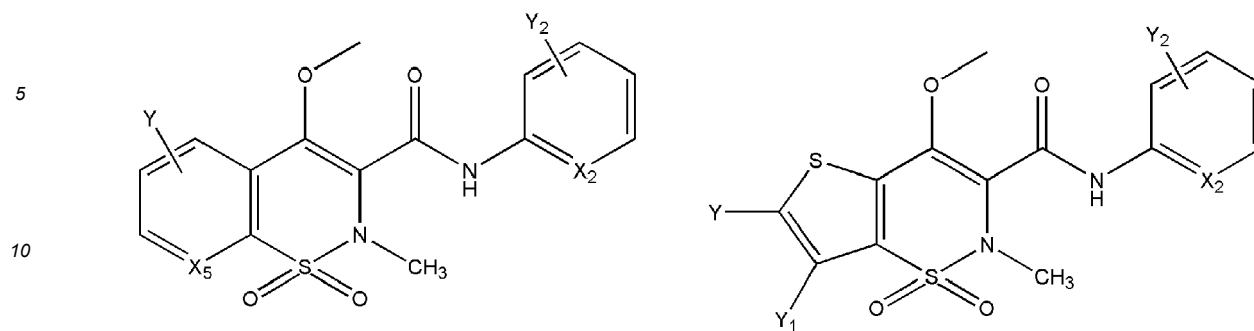
[Chem.30]
