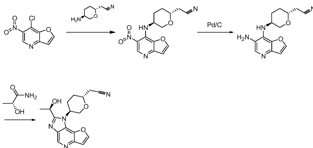
Compound I
