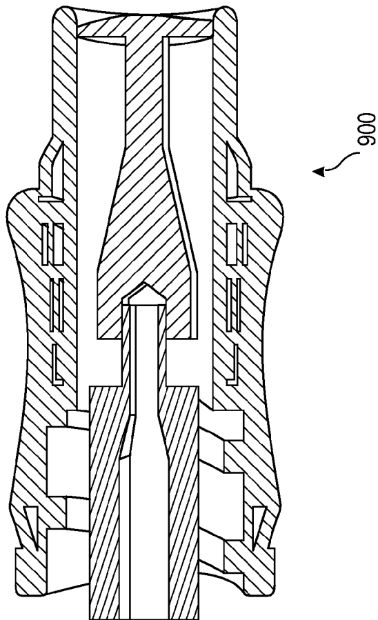
FIG. 38 (PRIOR ART)
