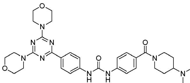
1-(4-[[4-(dimethylamino)piperidin-1-yl] carbonyl]phenyl)-3-[4-(4,6-dimorpholin-4-yl- 1,3,5-triazin-2-yl)phenyl]urea
