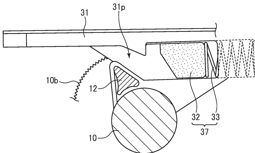
ENLARGED A-A CROSS SECTION
