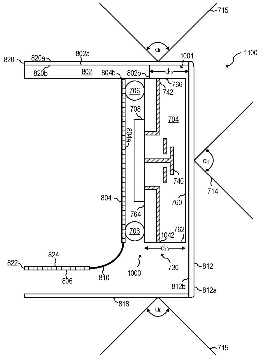
cross-section view
