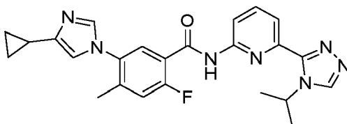
Compound I
