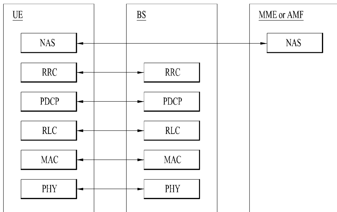
(b) Control Plane Protocol Stack
