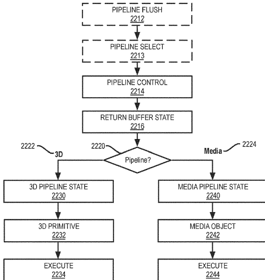
FIG. 22B GRAPHICS PROCESSOR COMMAND SEQUENCE 2210
