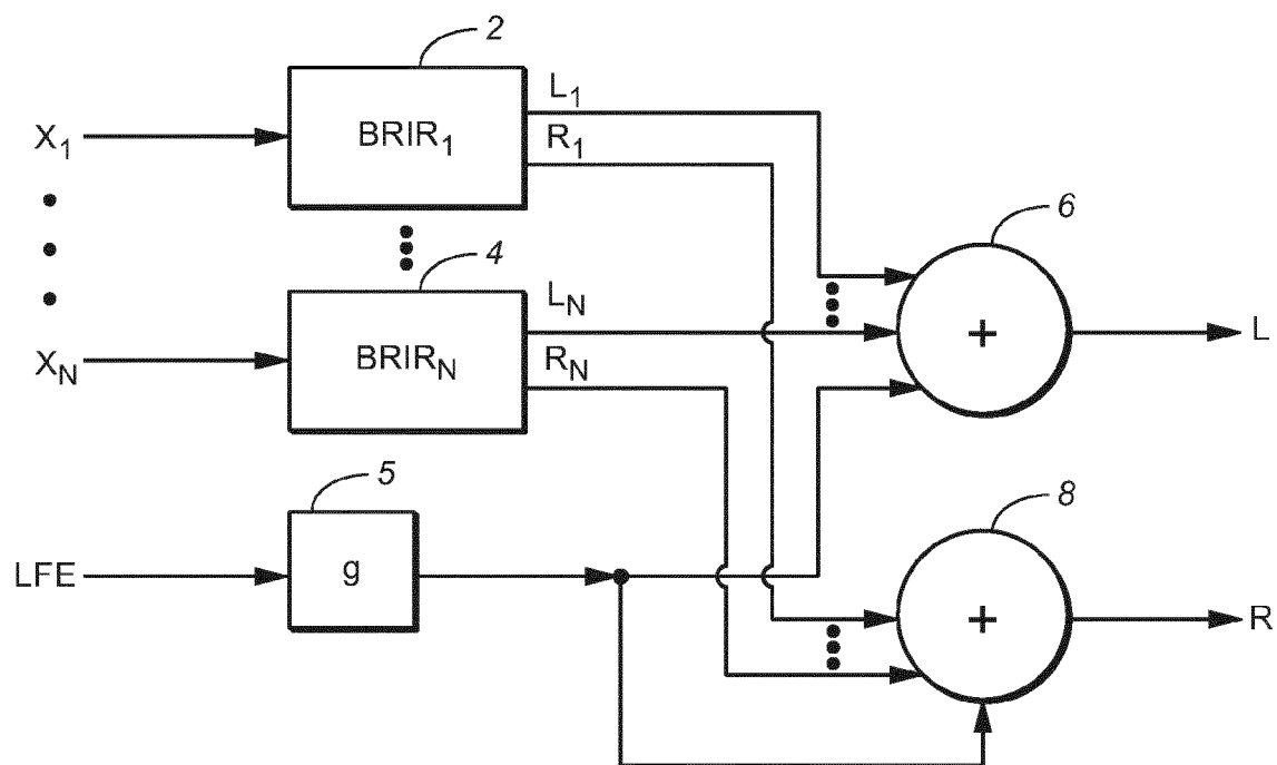
FIG. 1 (PRIOR ART)
