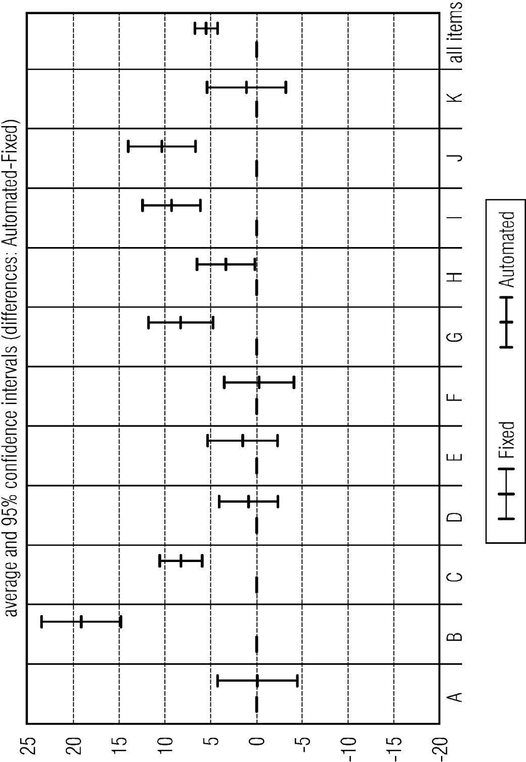
Fig. 16 DIFFERENCE MUSHRA SCORES COMPARING PROPOSED AUTOMATED AGAINST FIXED IGF CONTROL
