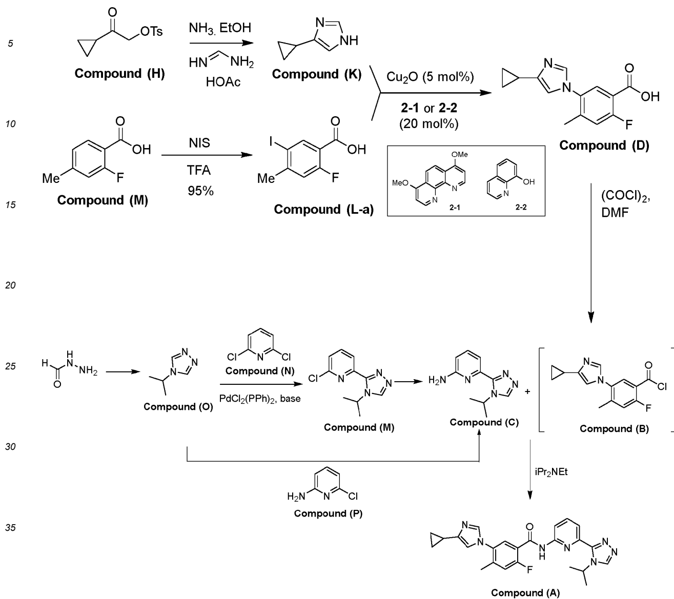
Scheme 2
