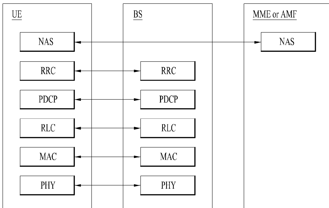
(b) Control Plane Protocol Stack
