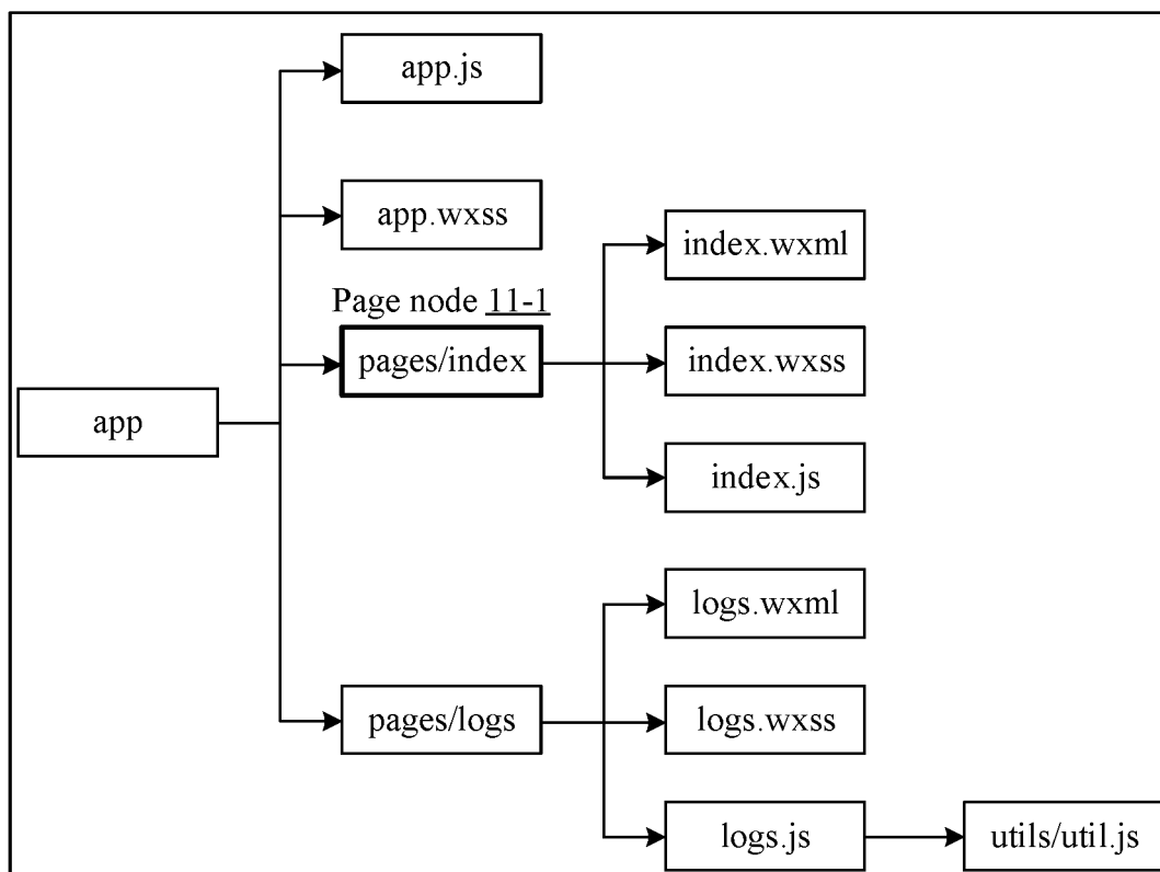
Code dependency relationship graph 9-1
