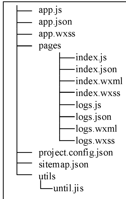
Code file directory structure information 8-1
