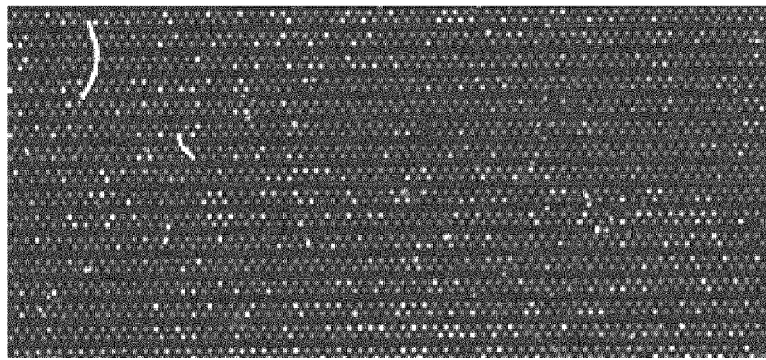
~1 copy/partition
