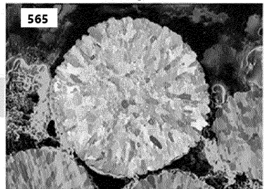
ML segmentation
