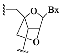
LNA (β-D-configuration) bridge = 4'-CH 2 -O-2'
