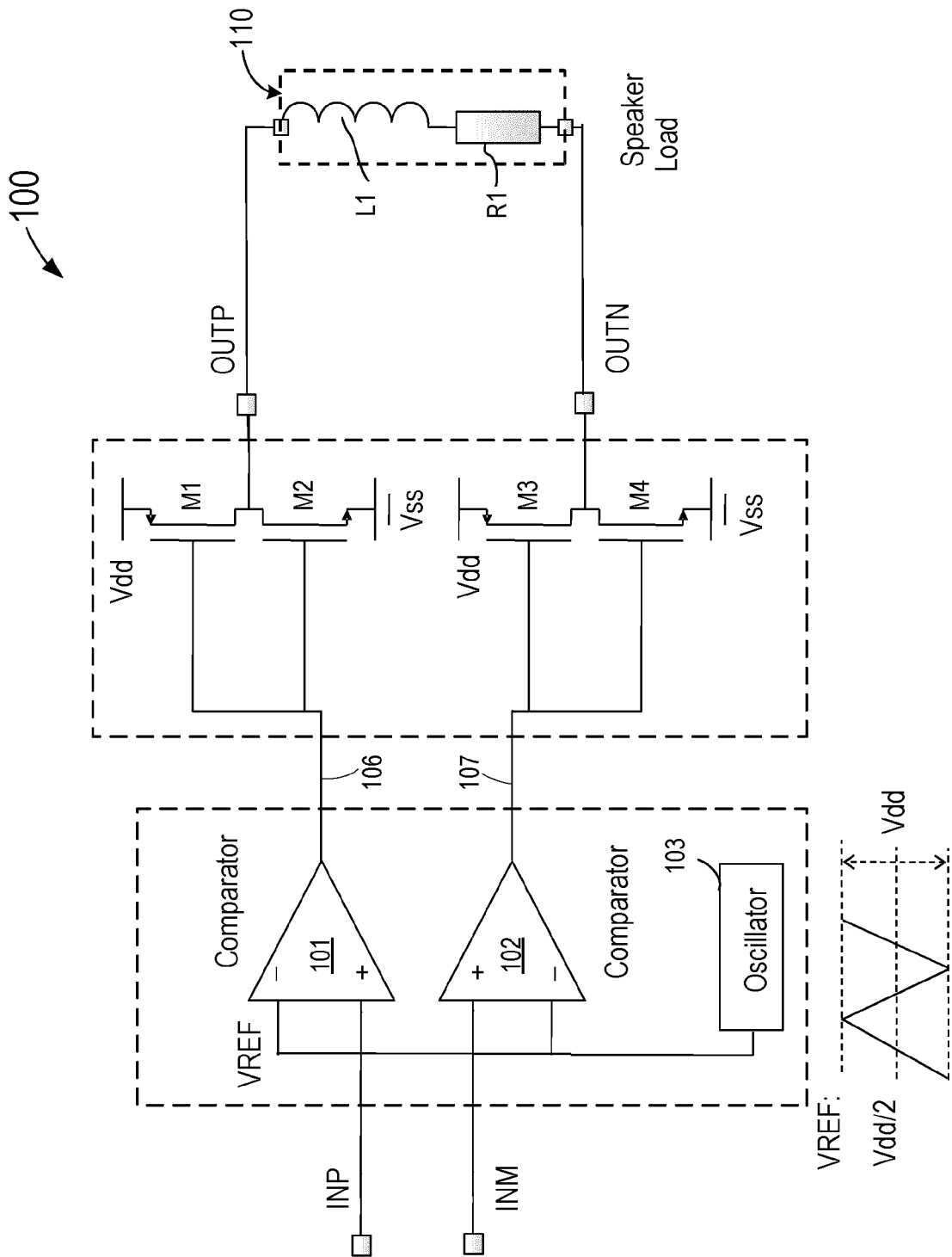
FIG. 1 (Prior Art)
