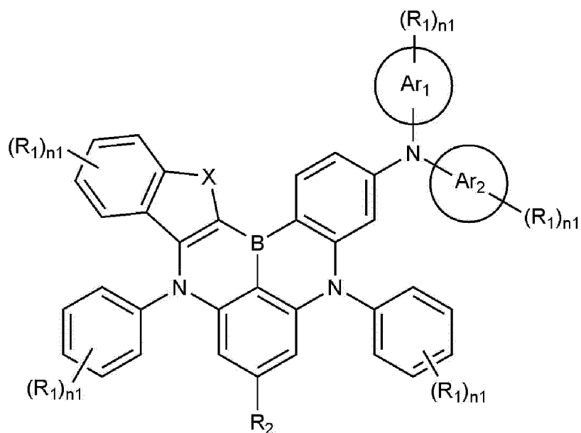
[Chemical Formula 2]
