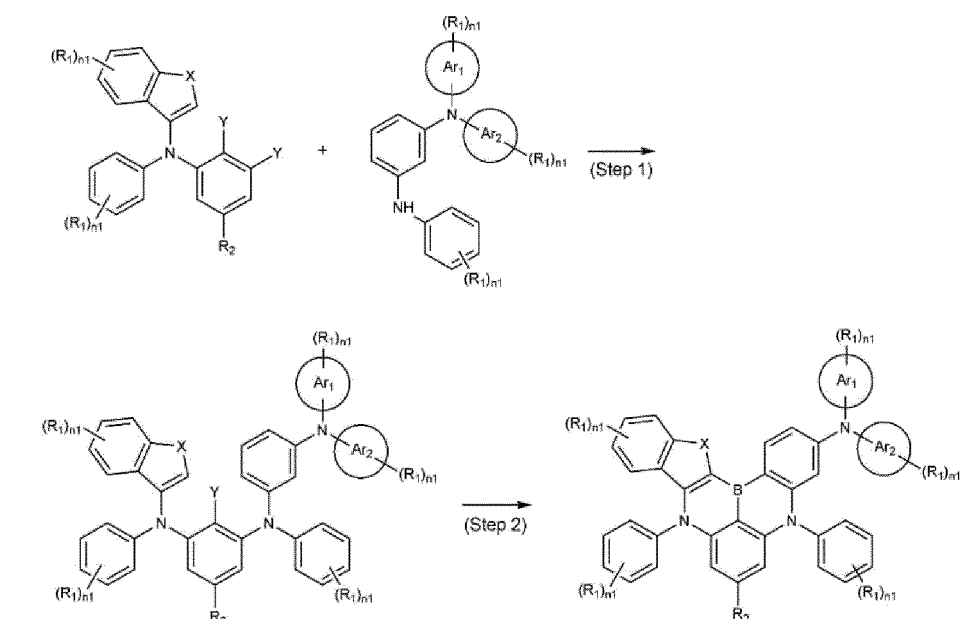
[Reaction Scheme 2]
