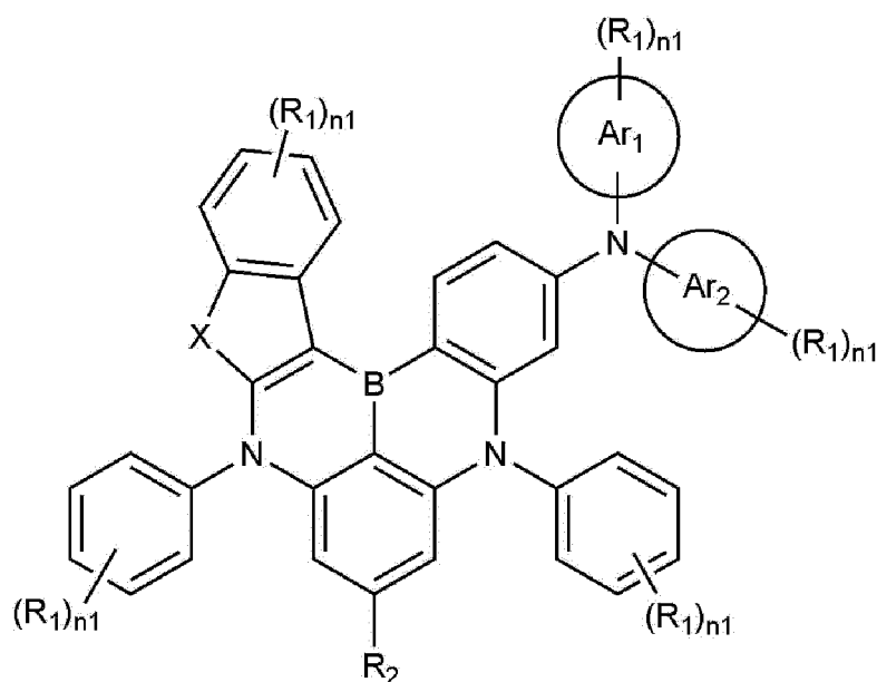
[Chemical Formula 2]
