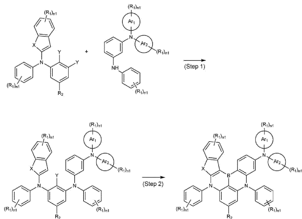
[Reaction Scheme 2]
