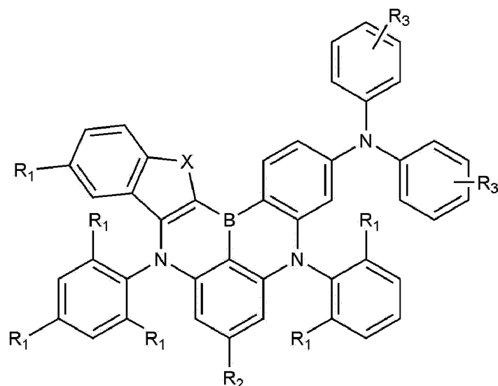
[Chemical Formula 1-1]
