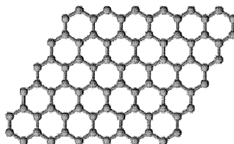
Graphene
