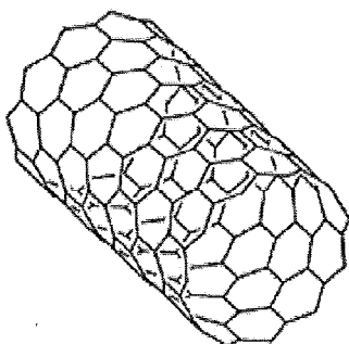
Carbon Nanotube
