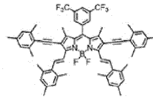
Compound (8)
