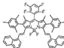
Compound (11)
