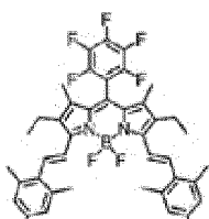
Compound (2)
