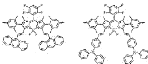
Compound (13) Compound (14)
