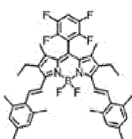
Comparative Compound (1)
