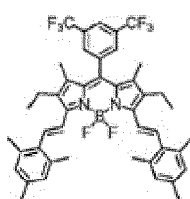
Compound (1)
