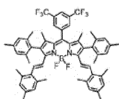
Compound (3)
