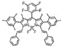
Compound (9)Compound (10)
