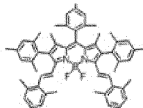
Compound (9)Compound (10)
