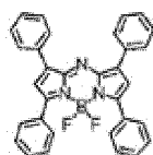
Comparative Compound (1)
