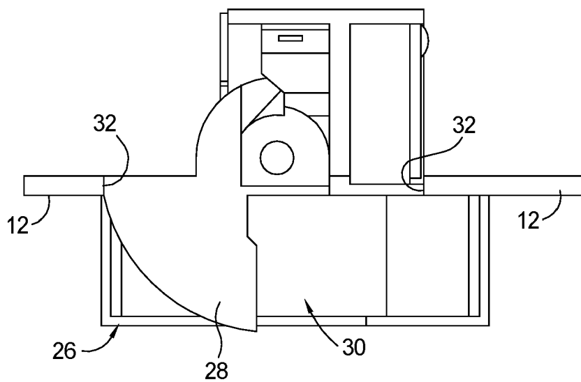
FIG. 4. PRIOR ART
