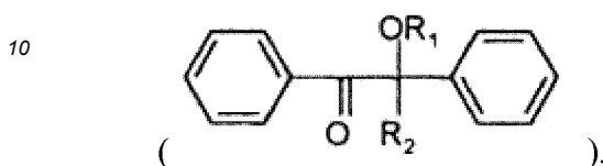
15 dialkoxyacetophenone
