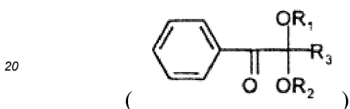
hydroxyalkyl ketone
