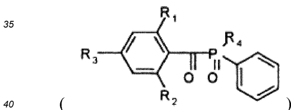
aminoketone
