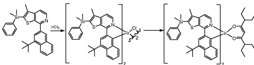
Inventive Compound 1
