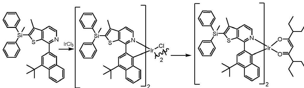
Inventive Compound 2
