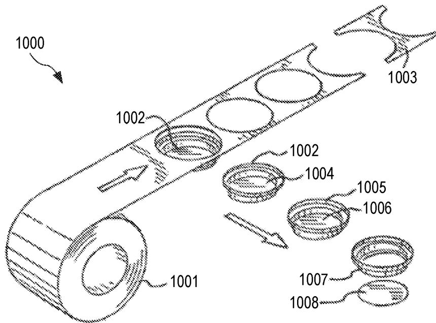
FIG. 10 (PRIOR ART)
