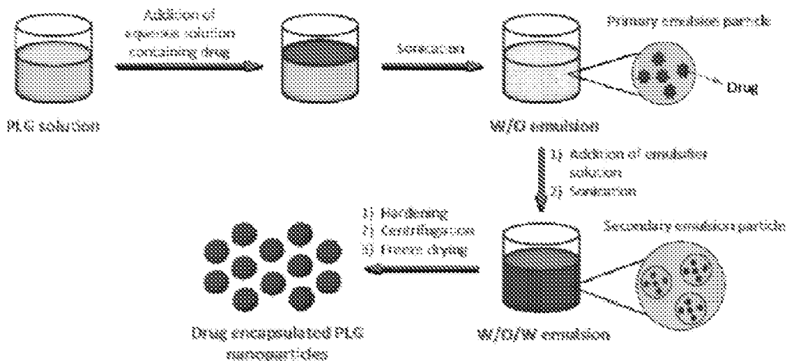
FIG. 2 Double Emulsion Process
