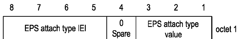
Figure 9.9.3.11.1: EPS attach type information element
