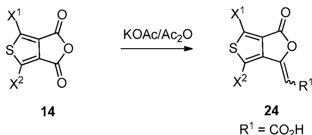
Scheme 10
