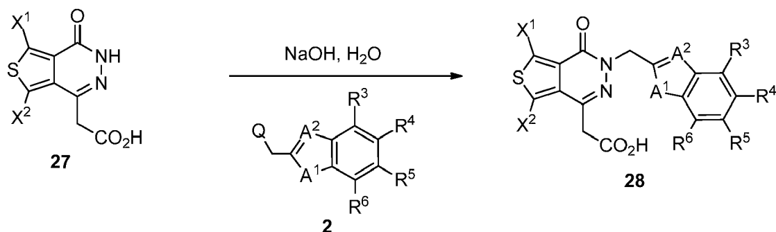
Scheme 17
