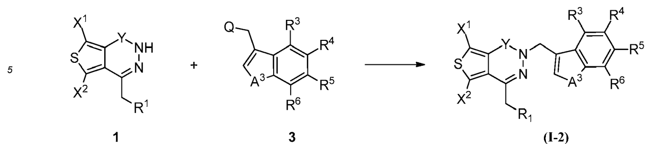
Scheme 2
