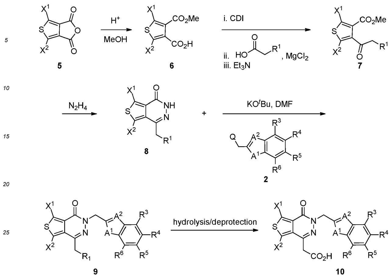
Scheme 4
