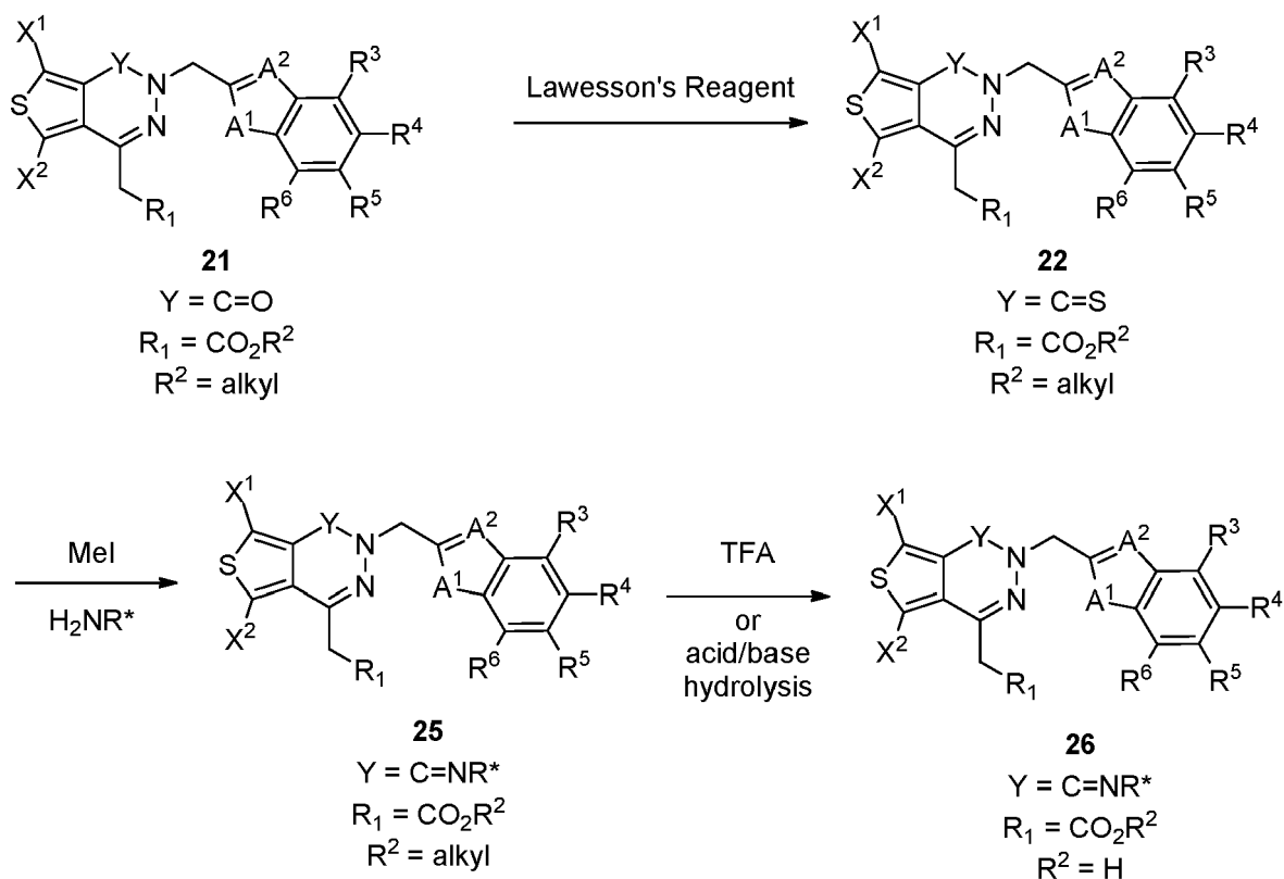
Scheme 16
