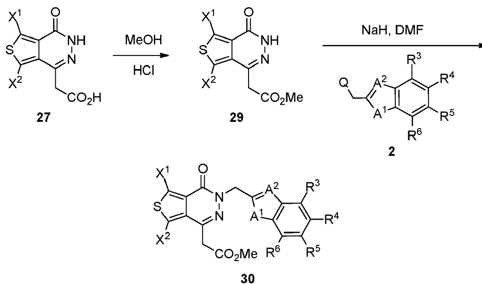
Scheme 18
