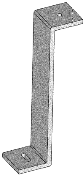
Query
