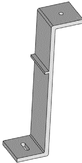
Closest (geometrically)
