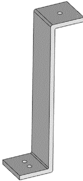
Closest (geometrically)
