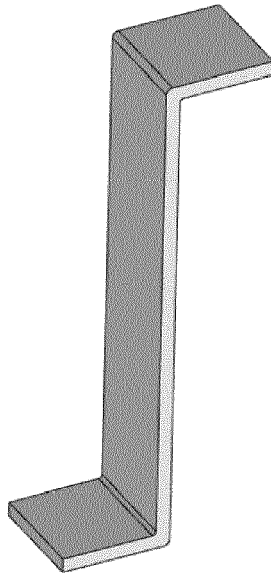
Closest (geometrically)
