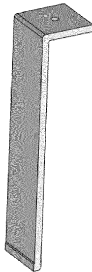
Closest (geometrically)
