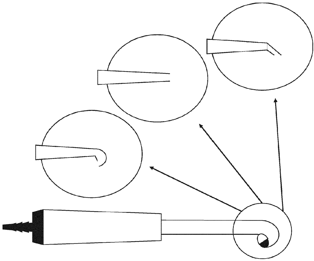
Interchangeable Tips
