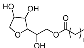
Sorbitan Laurate ( n = 10 )
