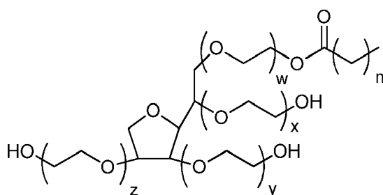
Polyoxyethylene Derivative of a Sorbitan Ester
