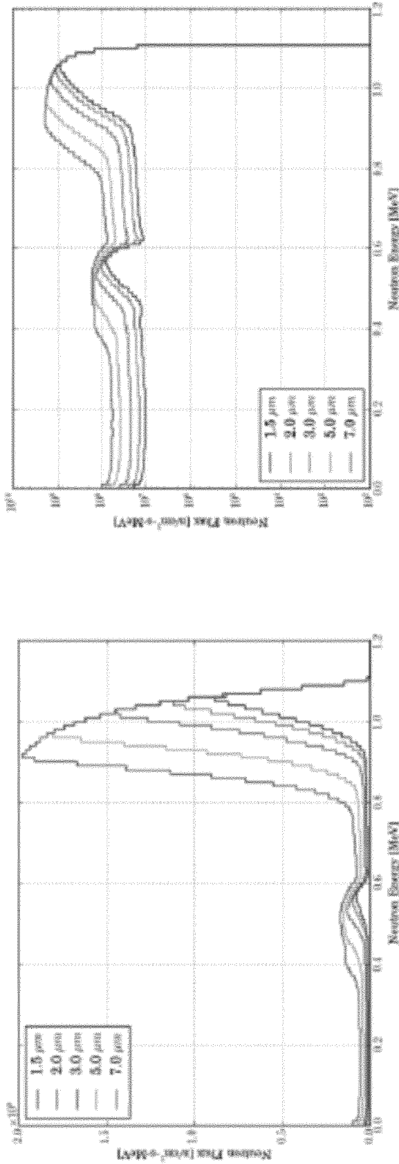
FIG. 12 1 MeV | p-LiF | 2 cm from target
