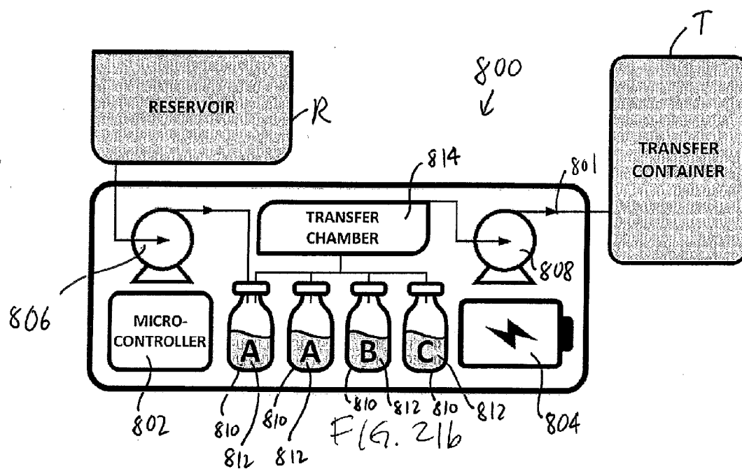
transfer device, powder w/ reconstitution, fully disposable
