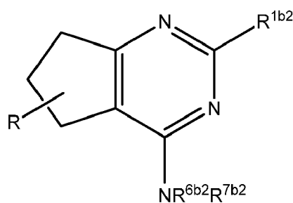
Formula VIIIb2
