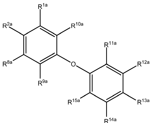
Formula XVIIa
