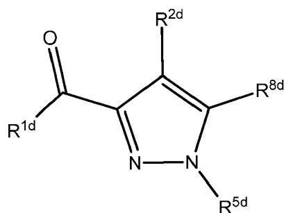
Formula IVd
