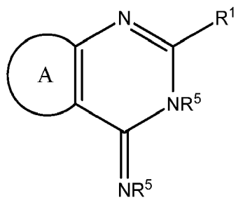
Formula VIIIa
