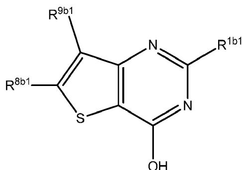
Formula VIb1
