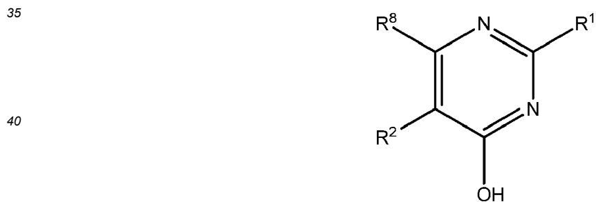
Formula VII
