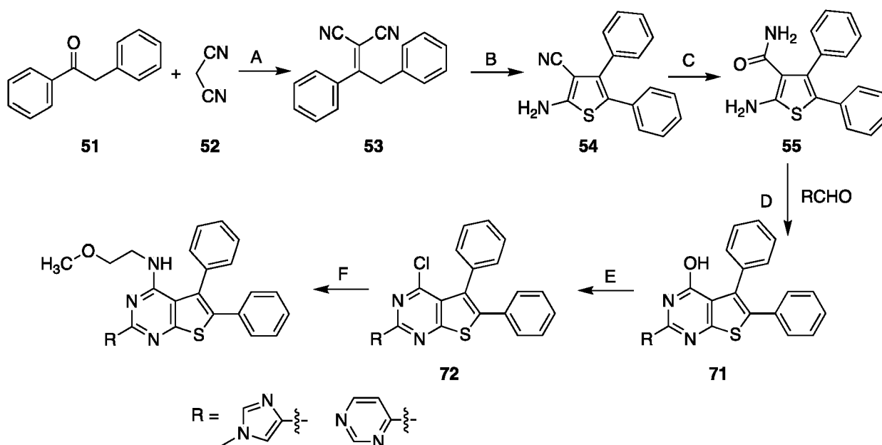
Scheme 16
