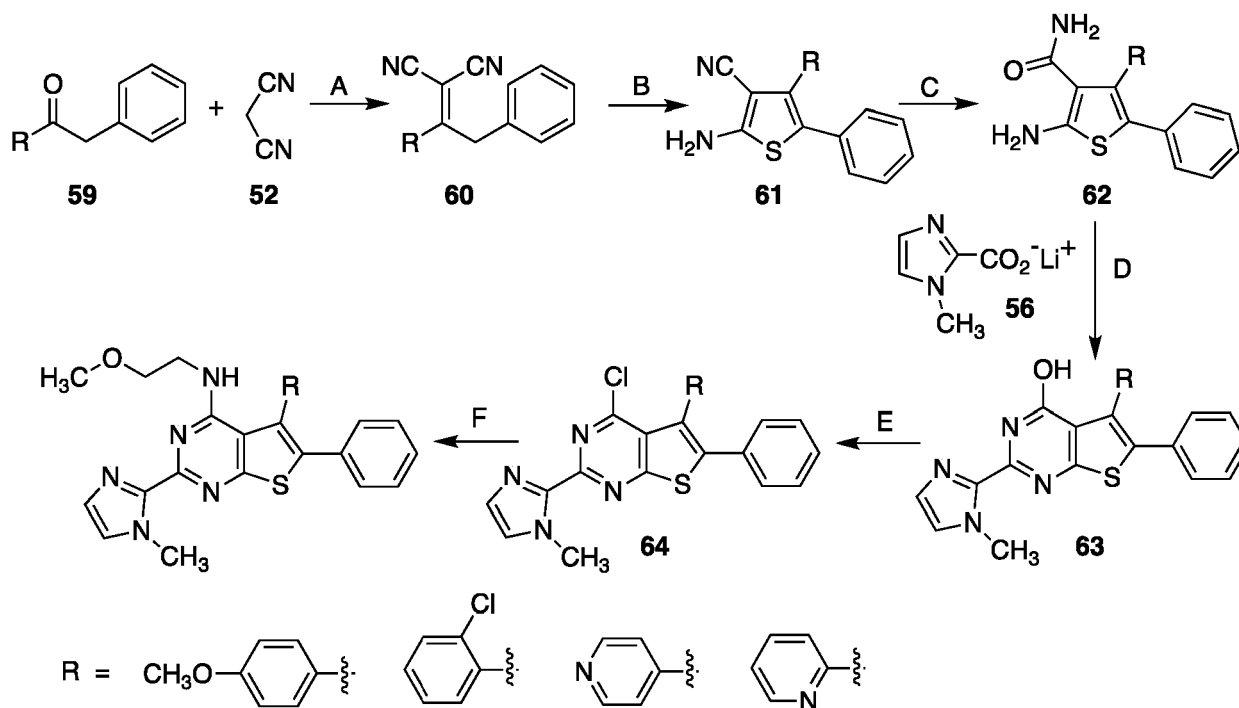
Scheme 14
