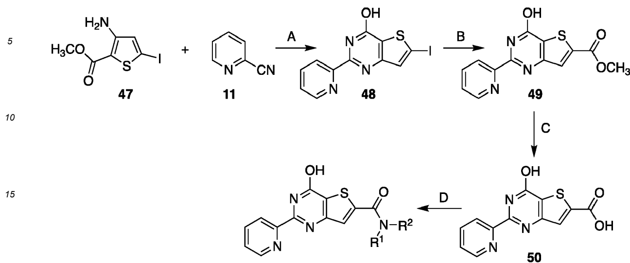
Scheme 11
