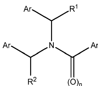
Formula XXII
