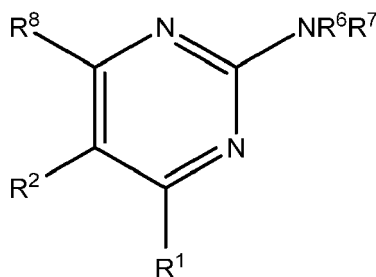
Formula X
