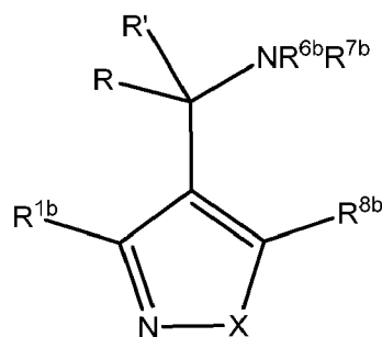
Formula IVb
