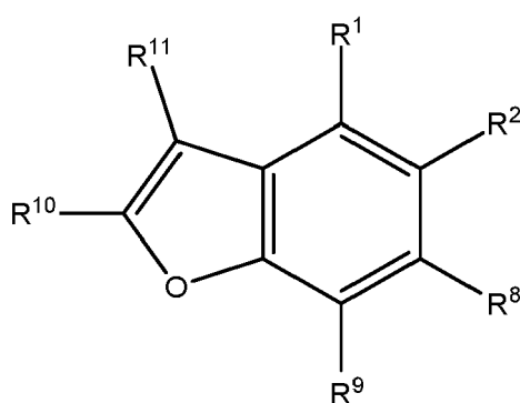
Formula XIII
