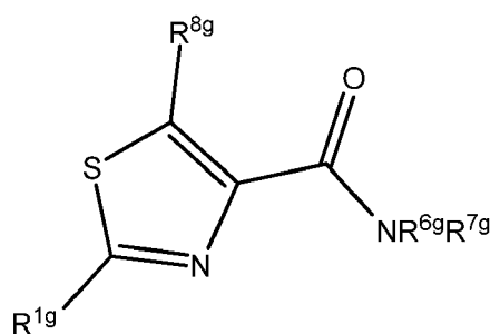
Formula IIIg
