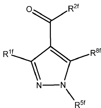
Formula IVf
