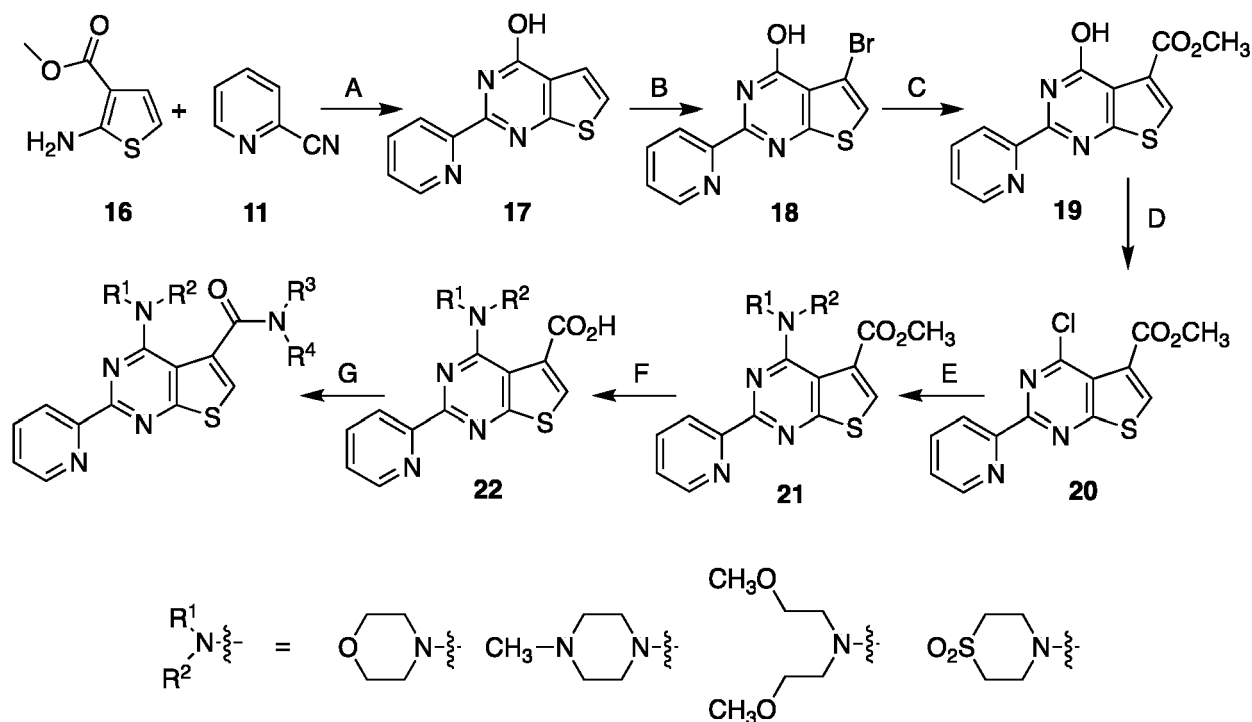
Scheme 5
