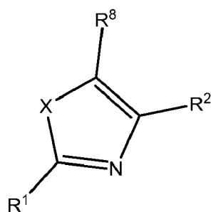
Formula III
