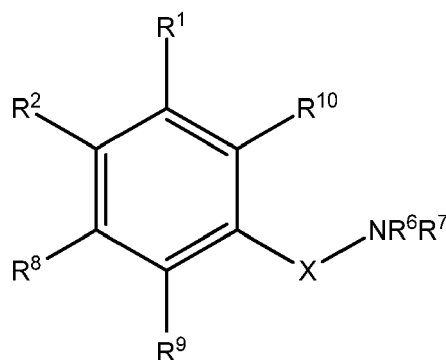
Formula XVIII
