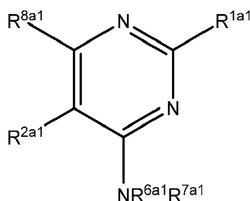
Formula IXa1
