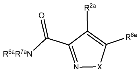
Formula IVa
