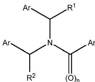
Formula XXII
