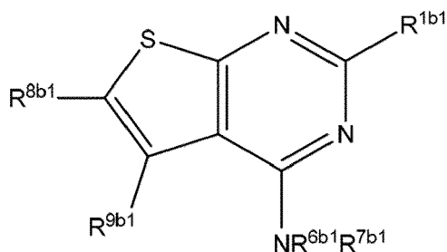
Formula VIIIb1,
