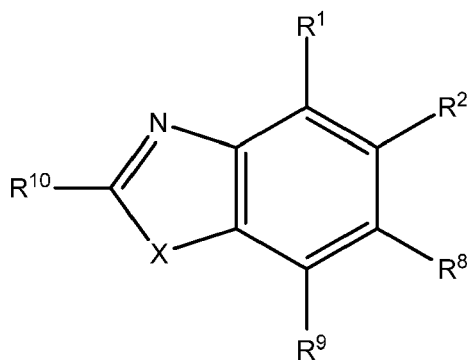
Formula XIV
