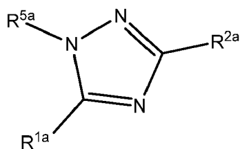
Formula IIa
