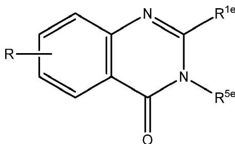
Formula VIe
