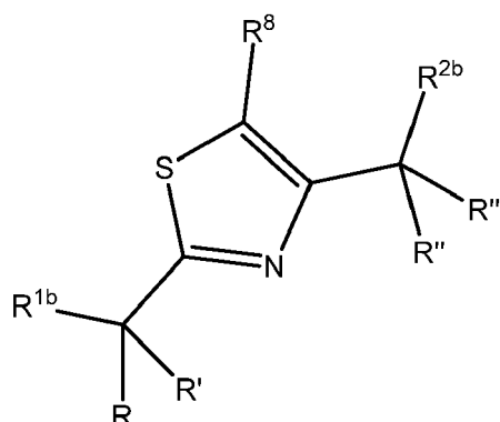
Formula IIIb
