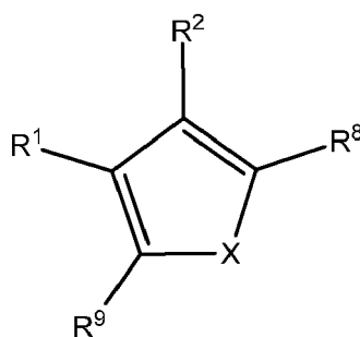
Formula V
