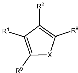
Formula V
