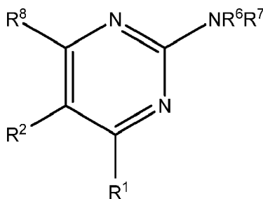
Formula X
