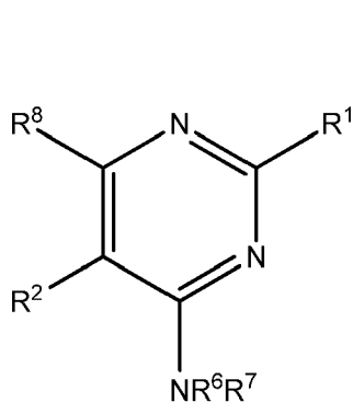
Formula IXa
