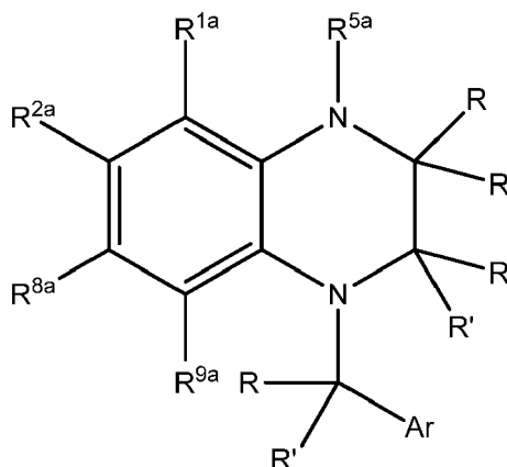
Formula XVIa
