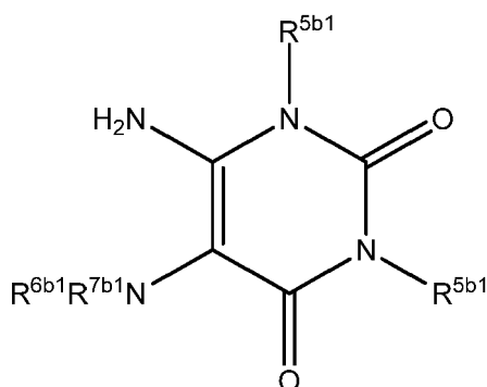
Formula IXb1
