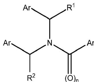
Formula XXII
