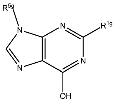
Formula VIg
