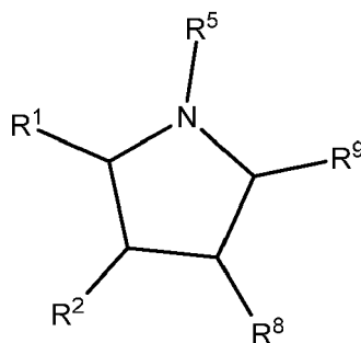
Formula XIX
