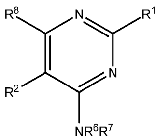
Formula IXa
