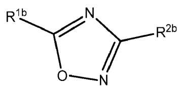
Formula XXb
