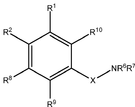
Formula XVIII
