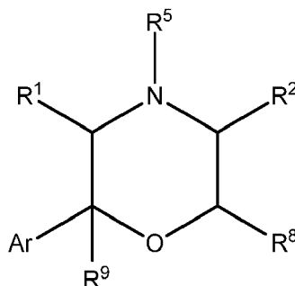
Formula XXI
