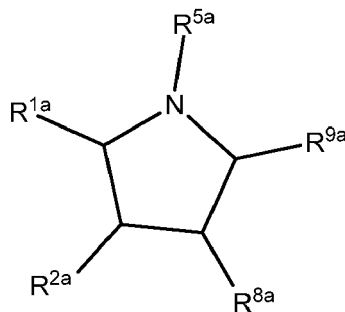
Formula XIXa
