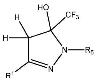
Formula XVa
