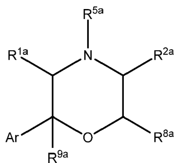
Formula XXIa
