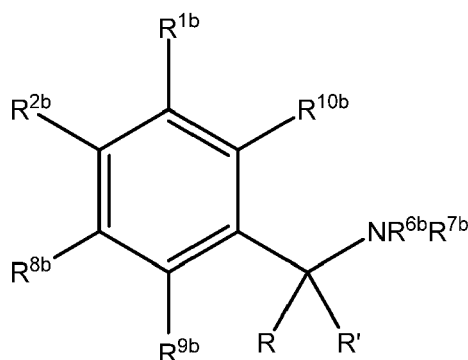
Formula XVIIIb
