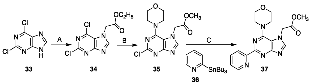
Scheme 9
