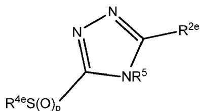
Formula Ia
