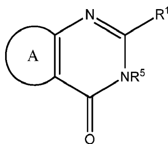
Formula VI
