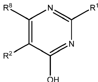
Formula VII
