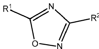
Formula XX
