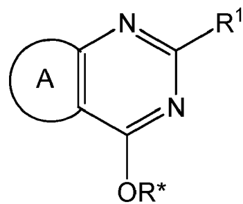
Formula VIa
