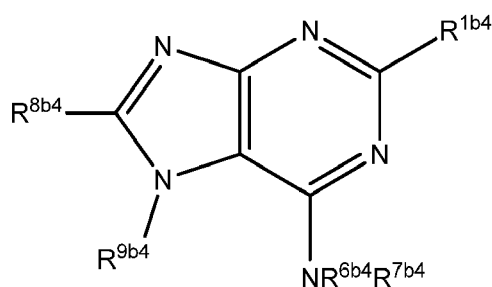
Formula VIIIb4
