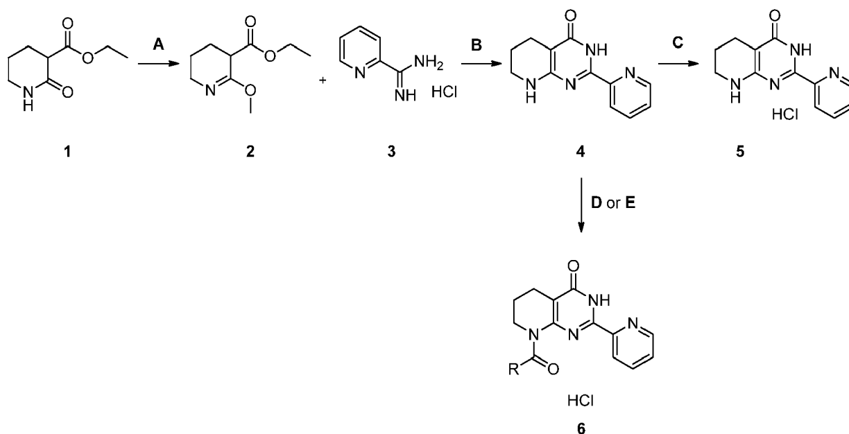
Scheme A
