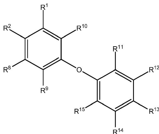
Formula XVII
