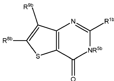
Formula VIb
