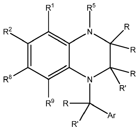
Formula XVI
