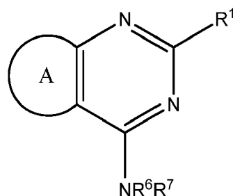
Formula VIIIb
