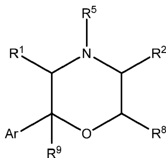
Formula XXI
