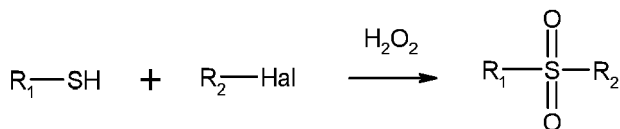
Reagent A
