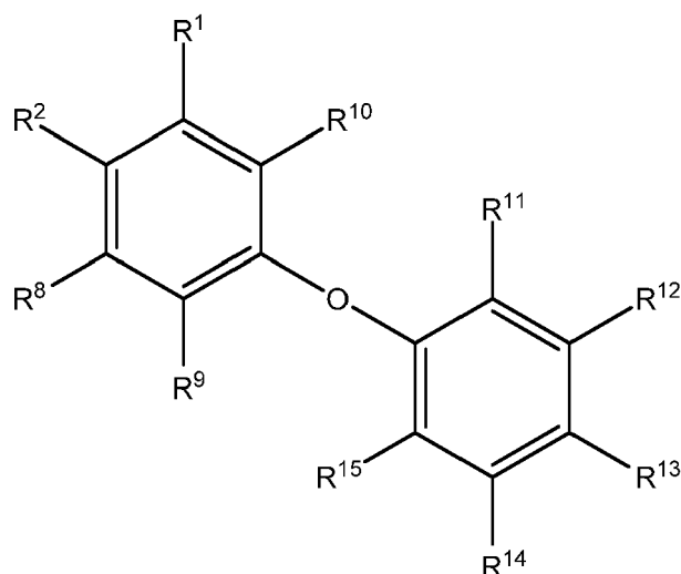
Formula XVII
