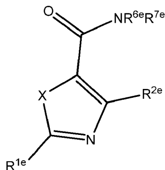
Formula IIIe
