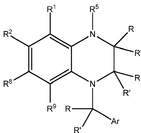
Formula XVI
