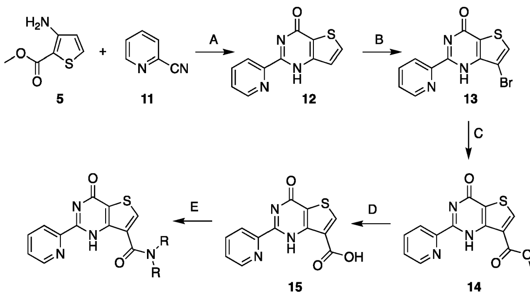
Scheme 3
