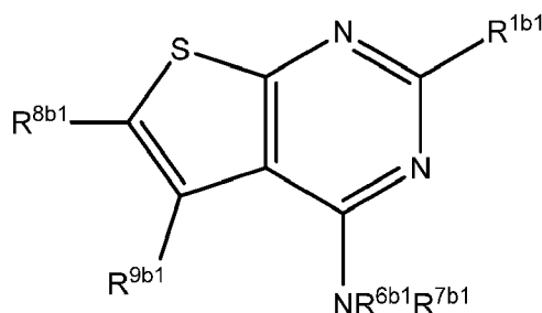
Formula VIIIb1
