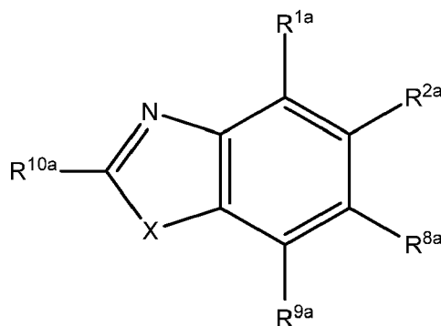
Formula XIVa
