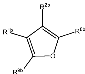
Formula Vb
