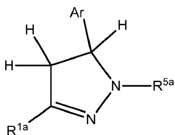
Formula XVb1
