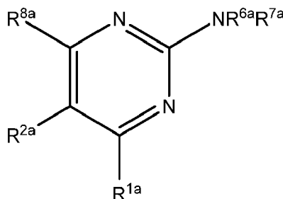
Formula Xa
