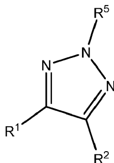
Formula XI
