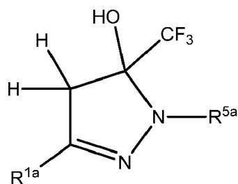
Formula XVa1
