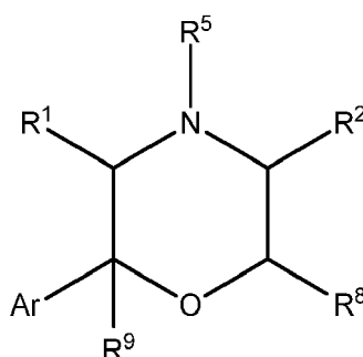
Formula XXI
