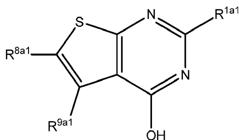
Formula VIa1
