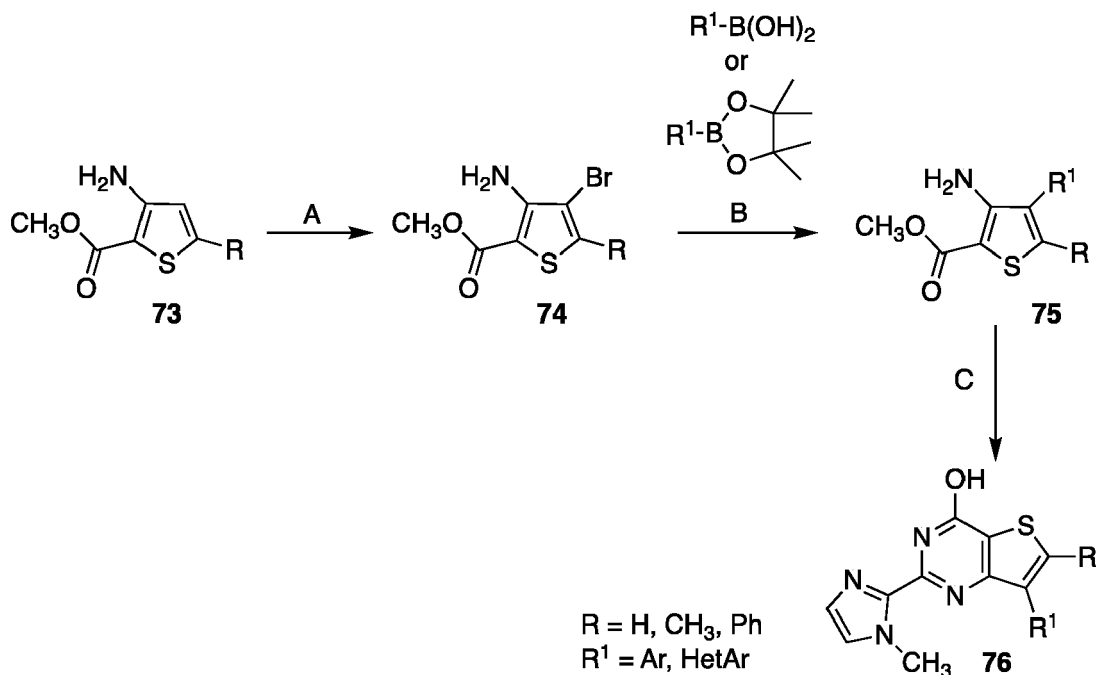
Scheme 17
