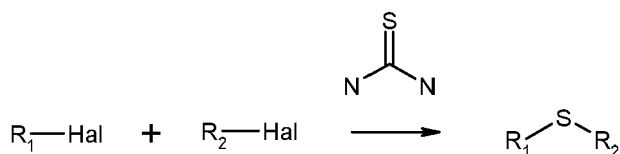
Reagent A
