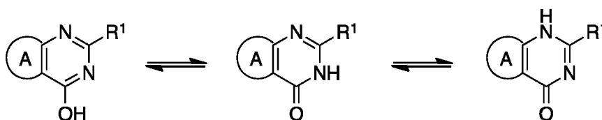
Formula VI
