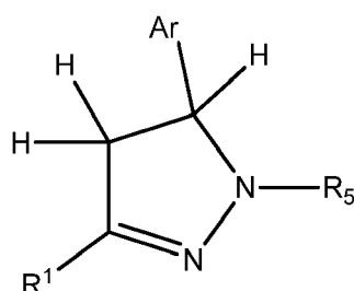
Formula XVb
