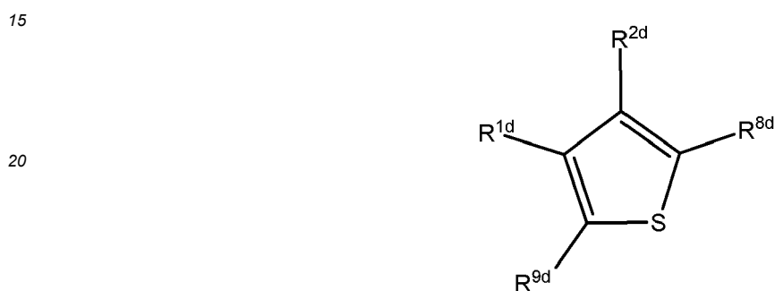
Formula Vd
