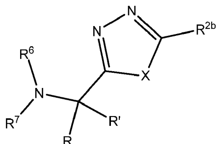
Formula Ib
