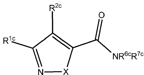
Formula IVc
