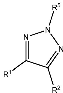
Formula XI
