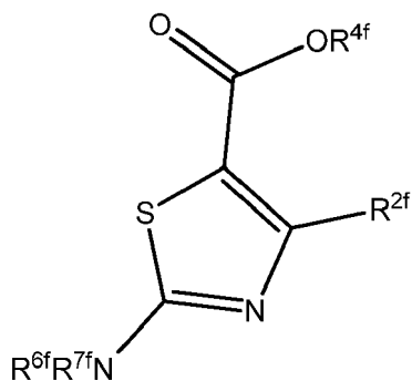
Formula IIIf
