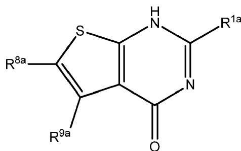
Formula VIa
