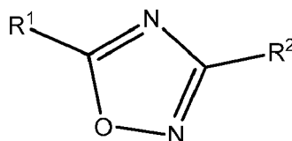
Formula XX
