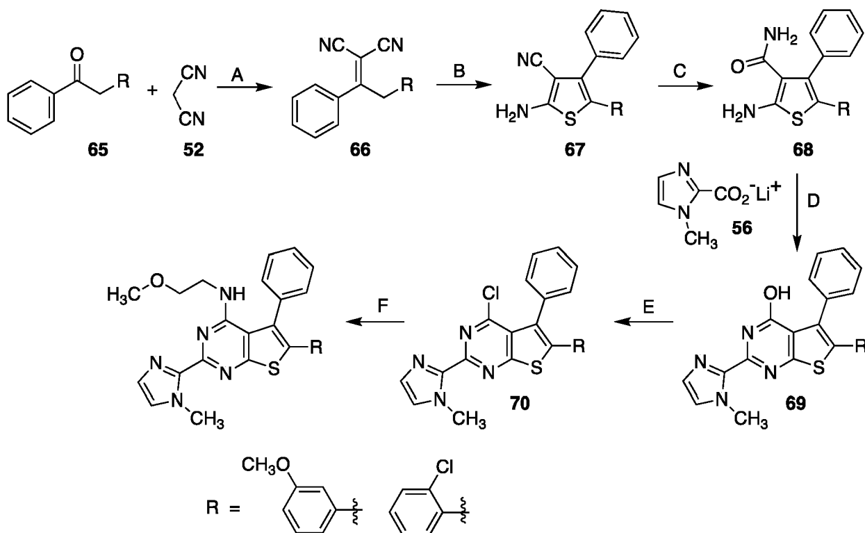
Scheme 15
