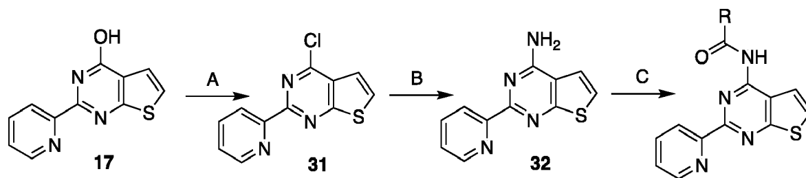
Scheme 8
