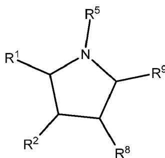
Formula XIX
