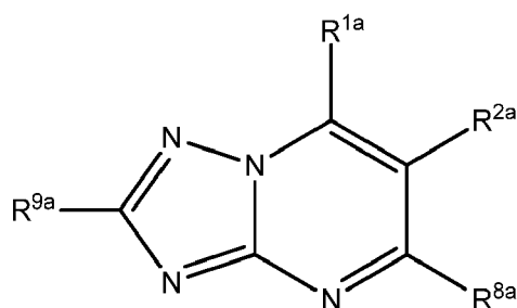
Formula XIIa
