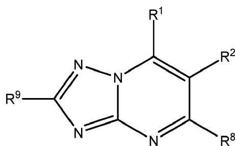
Formula XII
