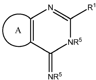
Formula VIIa
