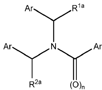
Formula XXIIa
