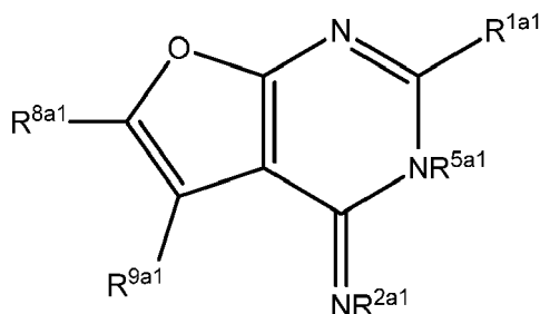
Formula VIIIa1
