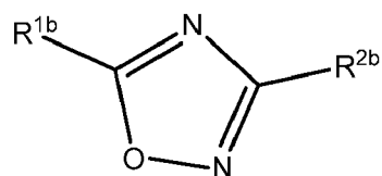
Formula XXc
