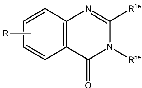
Formula VIe
