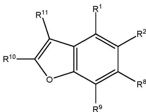
Formula XIII
