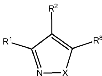
Formula IV
