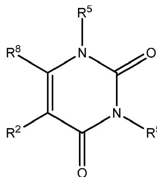
Formula IXb
