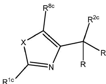
Formula IIIc
