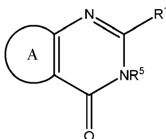
Formula VI
