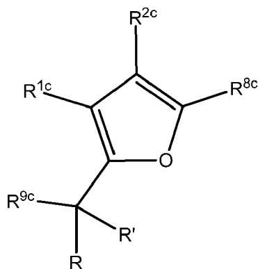
Formula Vc
