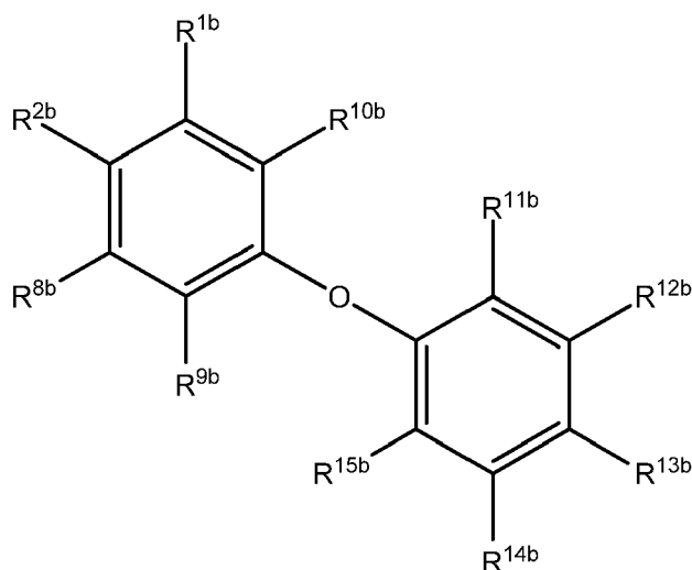
Formula XVIIb
