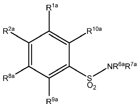
Formula XVIIIa
