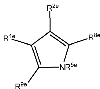
Formula Ve
