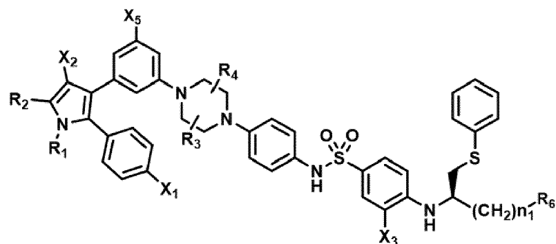
Formula (I)
