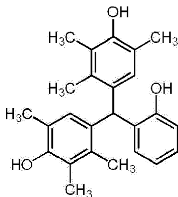
Polyhydric phenol compound (1)
