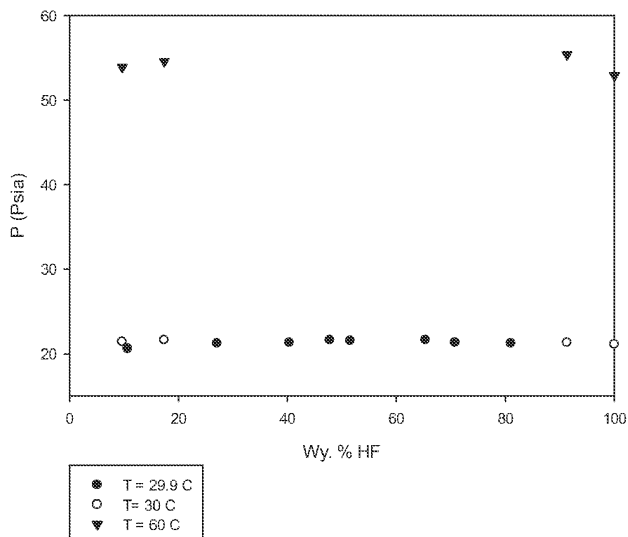
Figure 1: P-T-X of 240fa/HF
