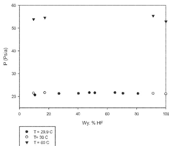
Figure 1: P-T-X of 240fa/HF
