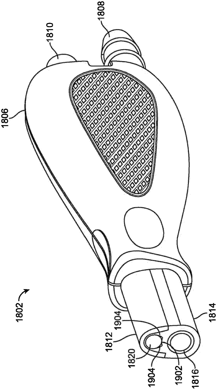
VIEW D-D
