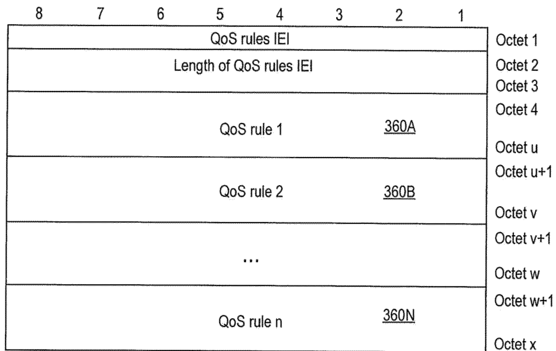
QoS rules information element
